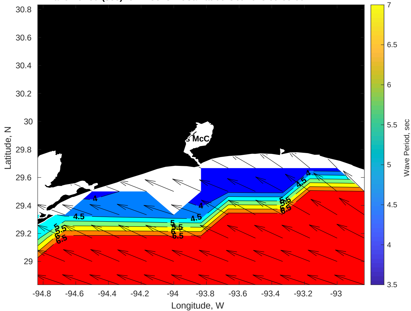
Wave Period (sec) for Brooks McCall at 06-Oct-2025 09:00:00
