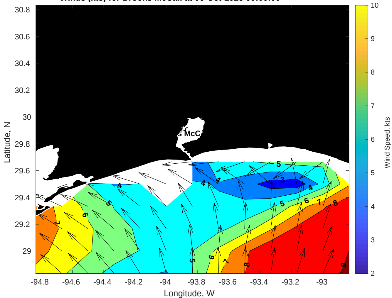
Winds (kts) for Brooks McCall at 06-Oct-2025 09:00:00
