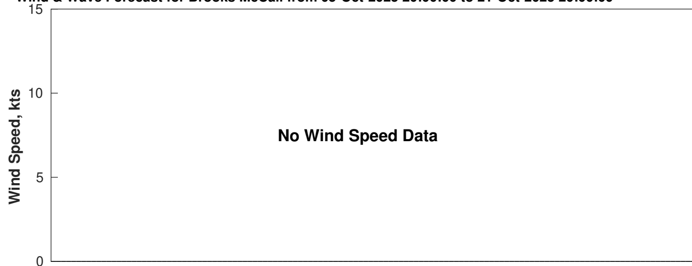
Wind & Wave Forecast for Brooks McCall from 05-Oct-2025 20:00:00 to 21-Oct-2025 20:00:00
