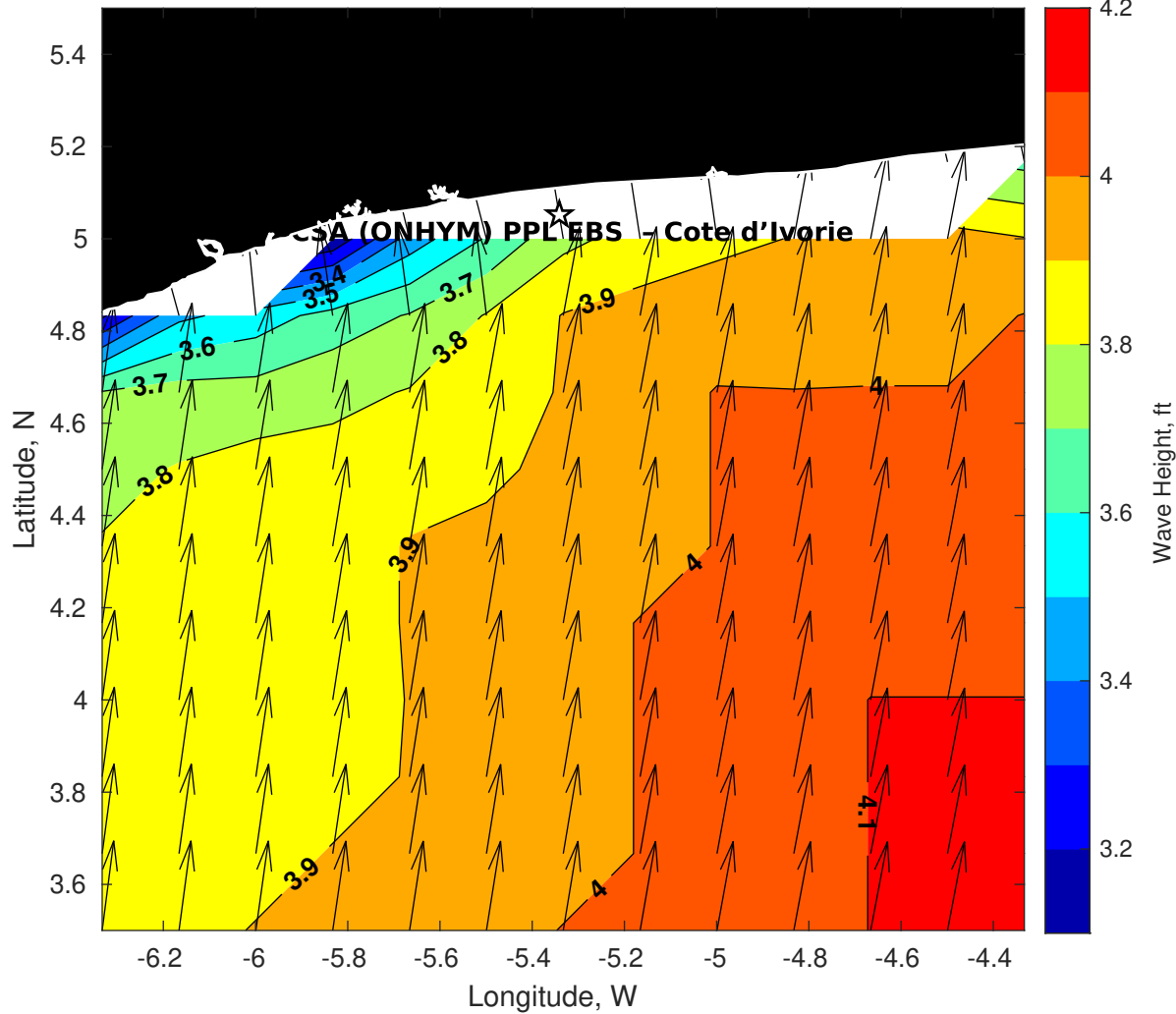
Wave Height (ft) for CSA (ONHYM) PPL EBS - Cote d'Ivoire at 06-Oct-2025 09:00:00
