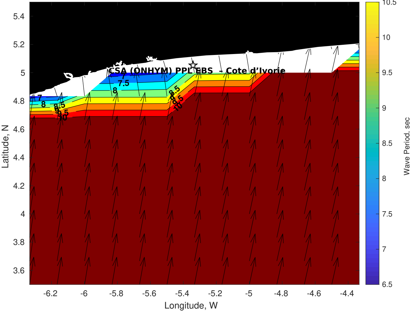
Wave Period (sec) for CSA (ONHYM) PPL EBS - Cote d'Ivoire at 06-Oct-2025 09:00:00
