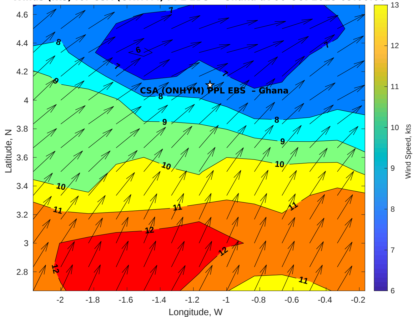
Winds (kts) for CSA (ONHYM) PPL EBS - Ghana at 06-Oct-2025 09:00:00
