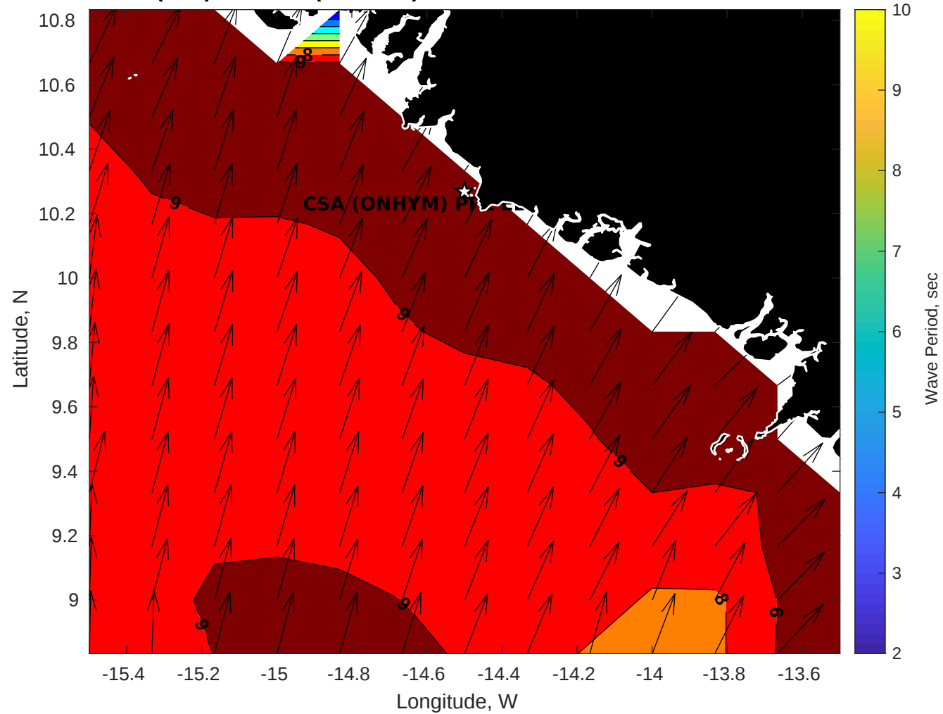
Wave Period (sec) for CSA (ONHYM) PPL EBS - Guinea at 06-Oct-2025 09:00:00
