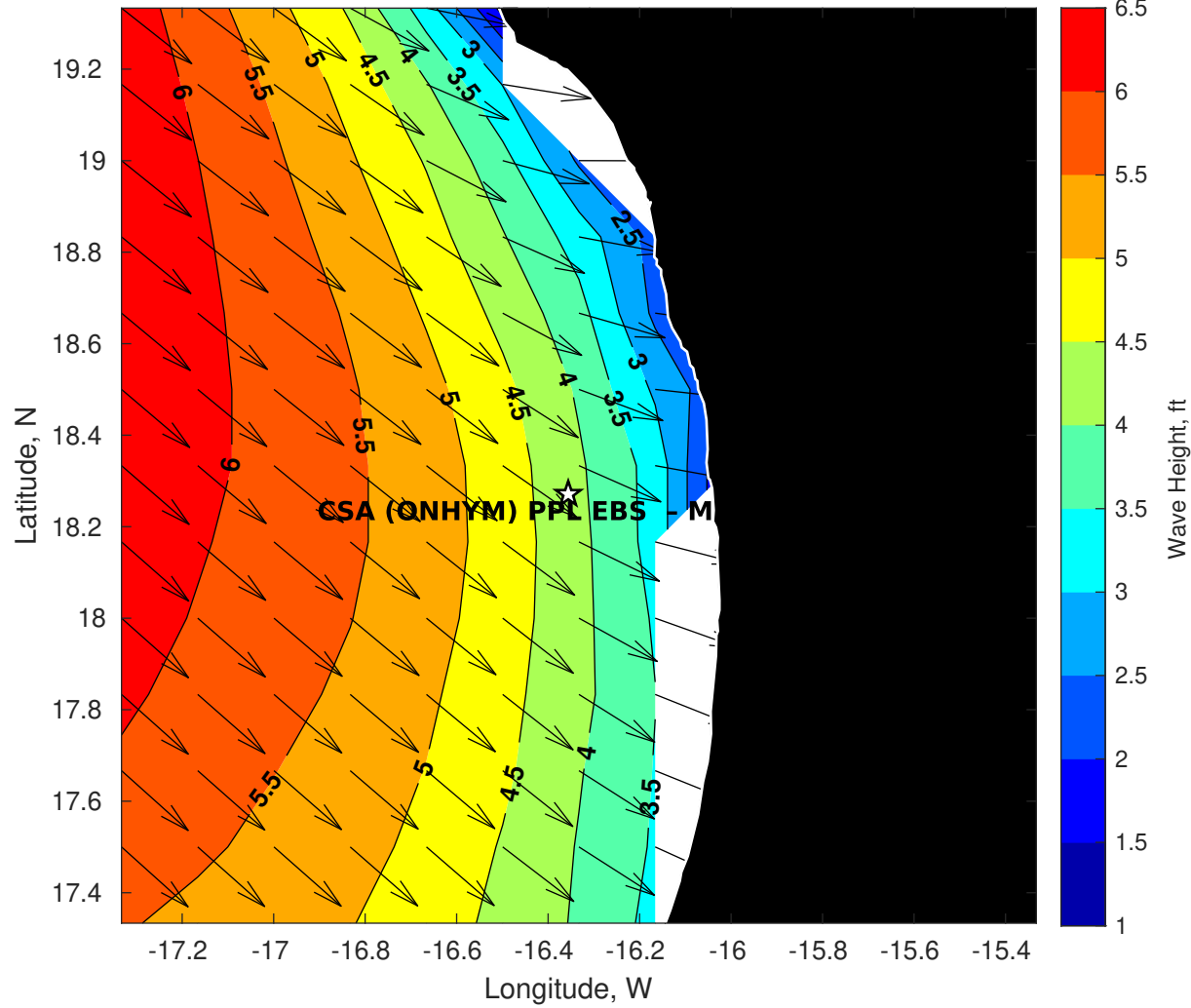
Wave Height (ft) for CSA (ONHYM) PPL EBS - Mauritania at 06-Oct-2025 09:00:00
