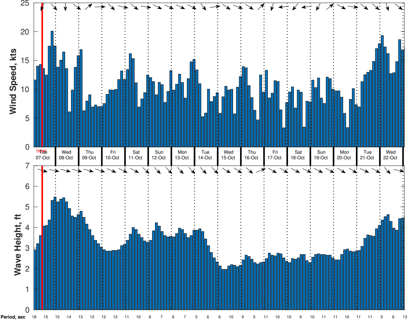
Wind & Wave Forecast for CSA (ONHYM) PPL EBS - Mauritania from 06-Oct-2025 01:00:00 to 22-Oct-2025 01:00:00
