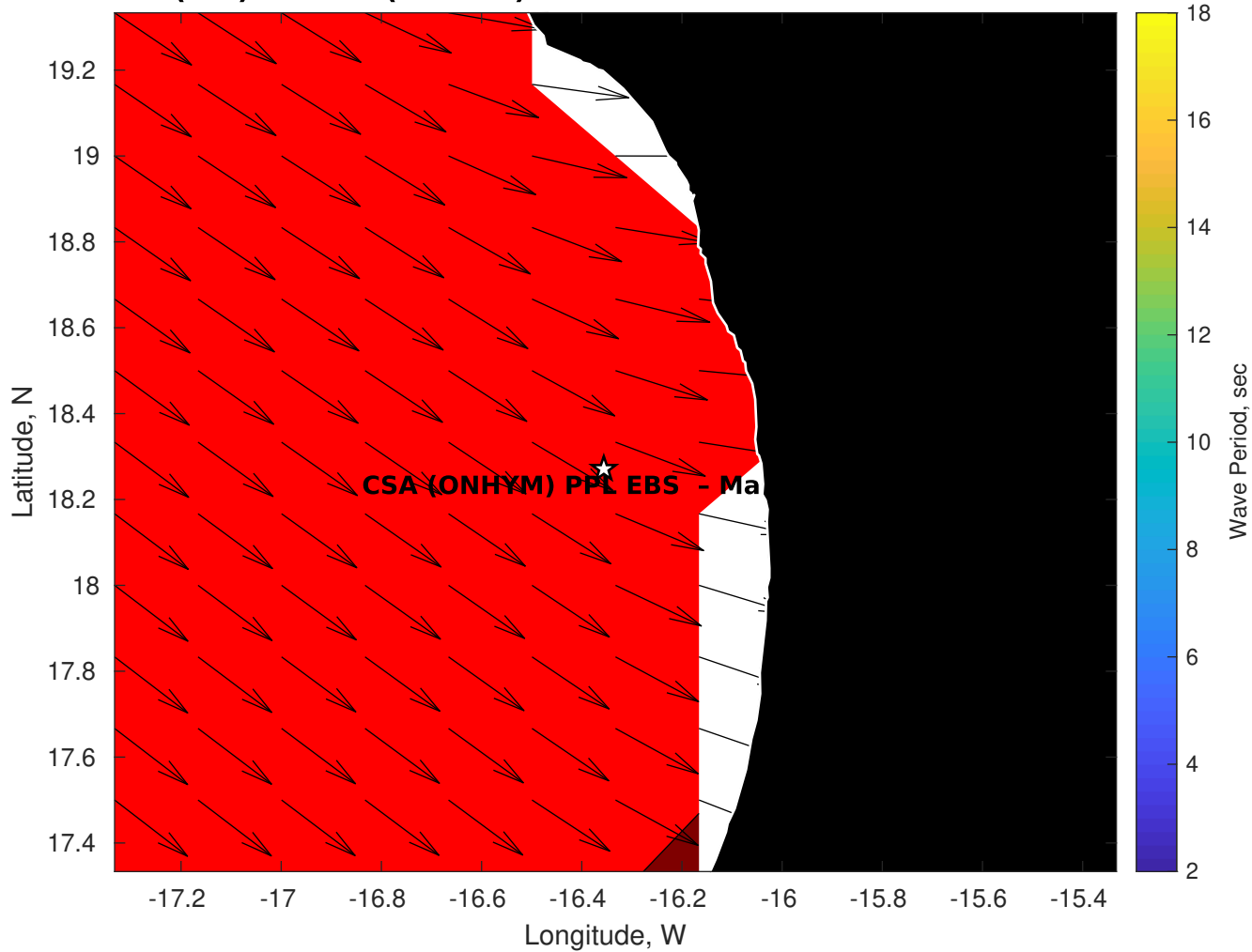
Wave Period (sec) for CSA (ONHYM) PPL EBS - Mauritania at 06-Oct-2025 09:00:00
