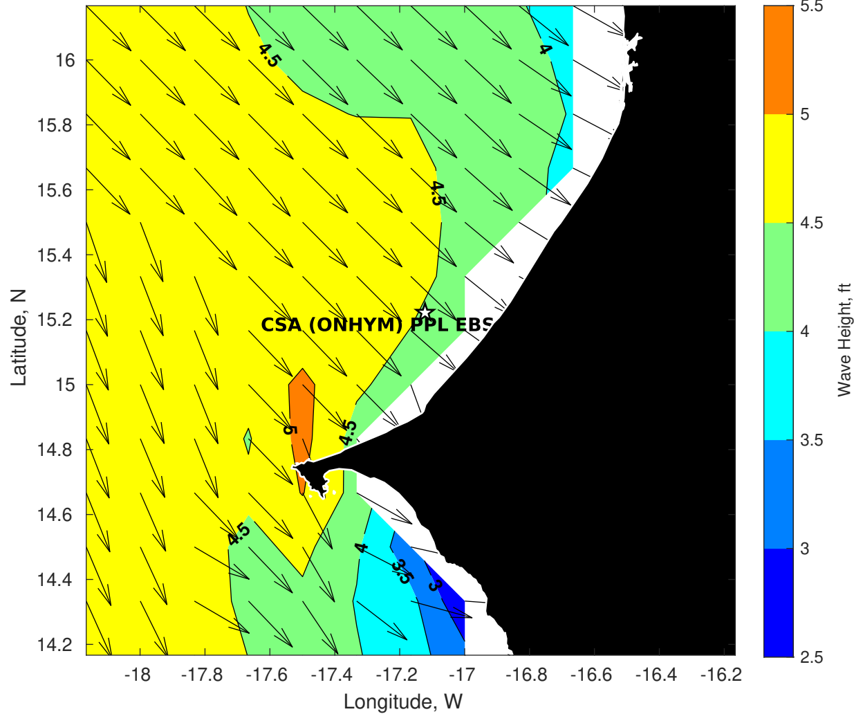
Wave Height (ft) for CSA (ONHYM) PPL EBS - Senegal at 06-Oct-2025 09:00:00
