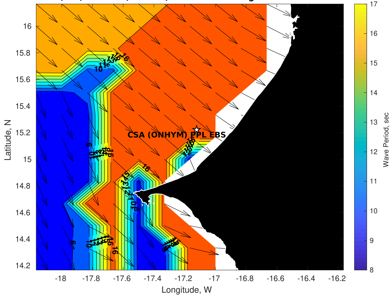
Wave Period (sec) for CSA (ONHYM) PPL EBS - Senegal at 06-Oct-2025 09:00:00
