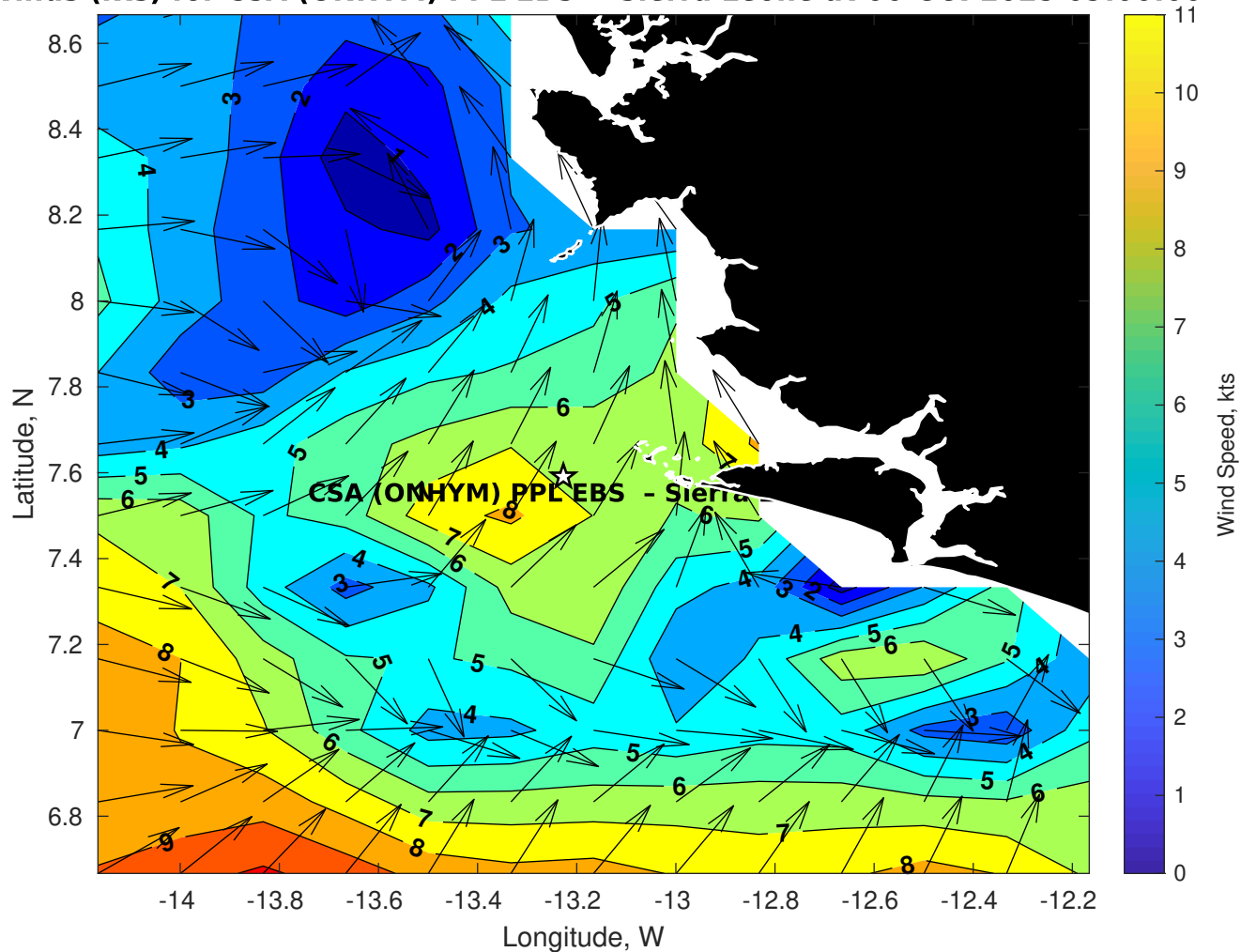
Winds (kts) for CSA (ONHYM) PPL EBS - Sierra Leone at 06-Oct-2025 09:00:00
