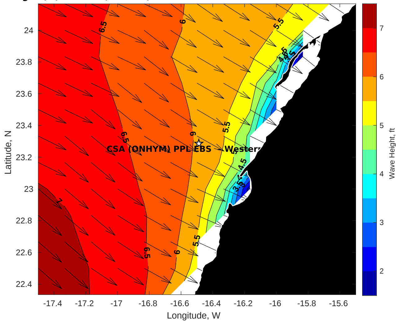
Wave Height (ft) for CSA (ONHYM) PPL EBS - Western Sahara at 06-Oct-2025 09:00:00
