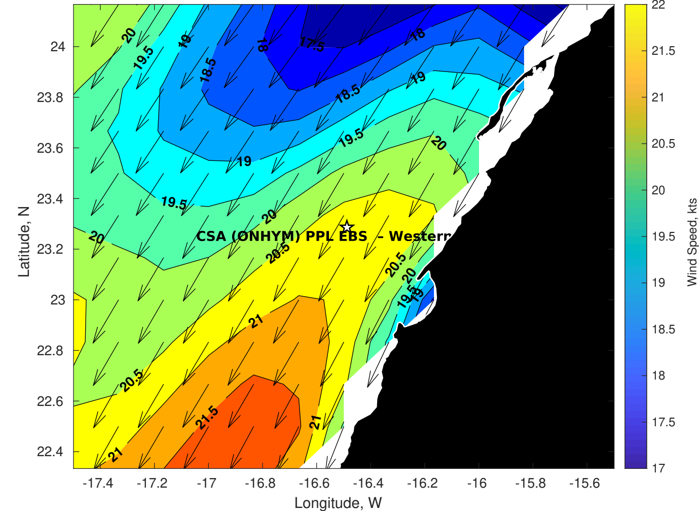
Winds (kts) for CSA (ONHYM) PPL EBS - Western Sahara at 06-Oct-2025 09:00:00
