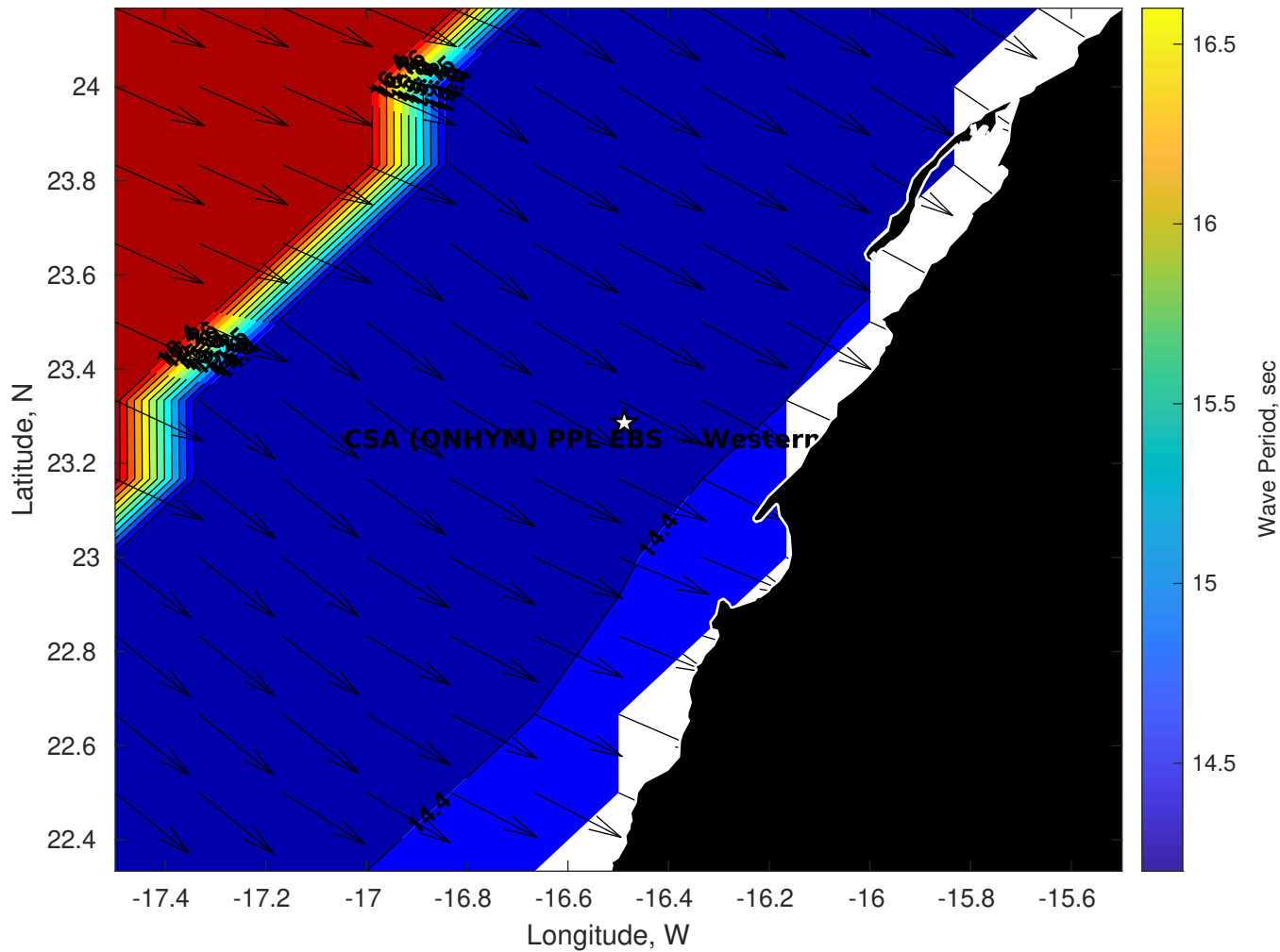
Wave Period (sec) for CSA (ONHYM) PPL EBS - Western Sahara at 06-Oct-2025 09:00:00
