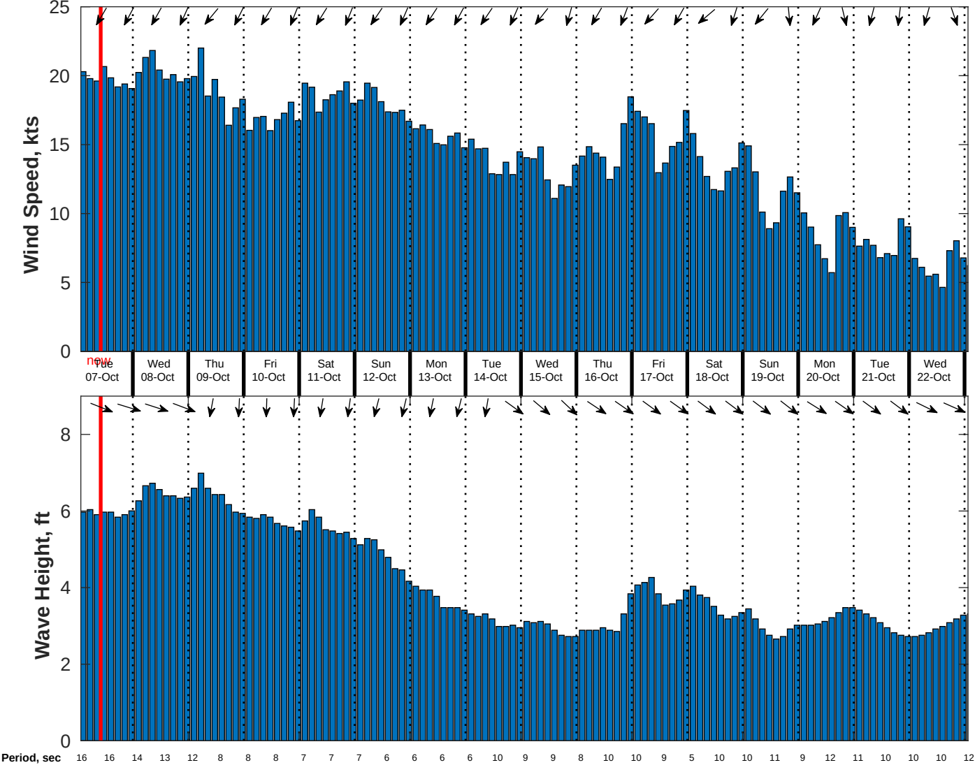
Wind & Wave Forecast for CSA (ONHYM) PPL EBS - Western Sahara from 06-Oct-2025 01:00:00 to 22-Oct-2025 01:00:00
