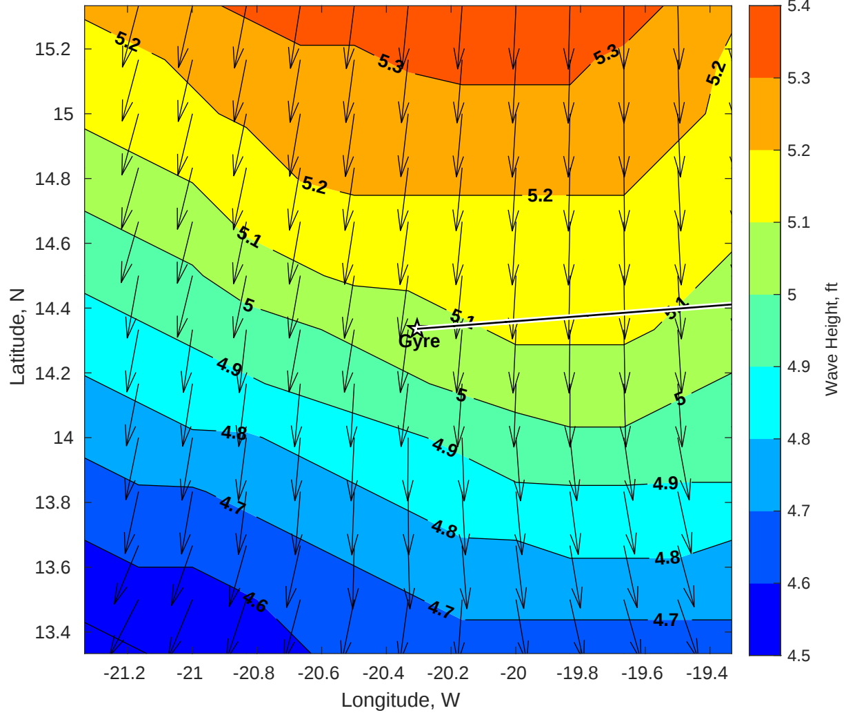
Wave Height (ft) for Gyre at 06-Oct-2025 09:00:00
