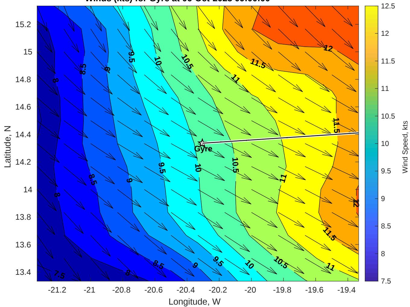
Winds (kts) for Gyre at 06-Oct-2025 09:00:00
