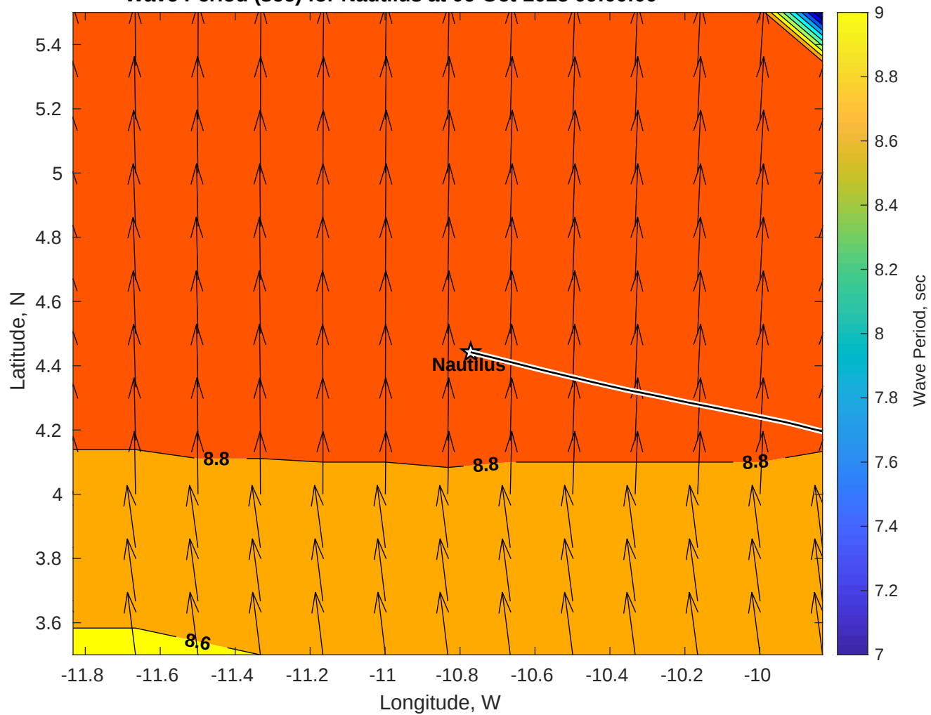
Wave Period (sec) for Nautilus at 06-Oct-2025 09:00:00
