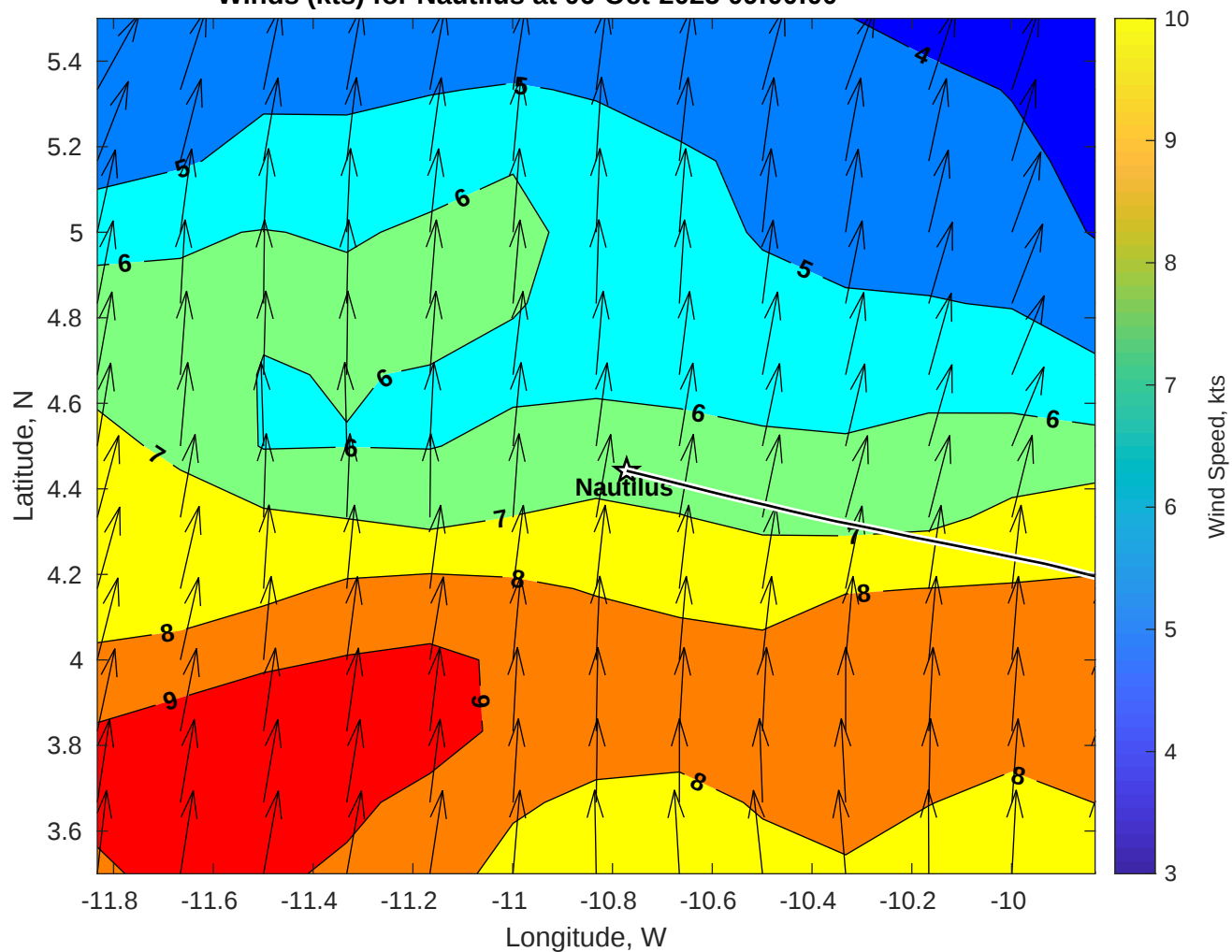
Winds (kts) for Nautilus at 06-Oct-2025 09:00:00
