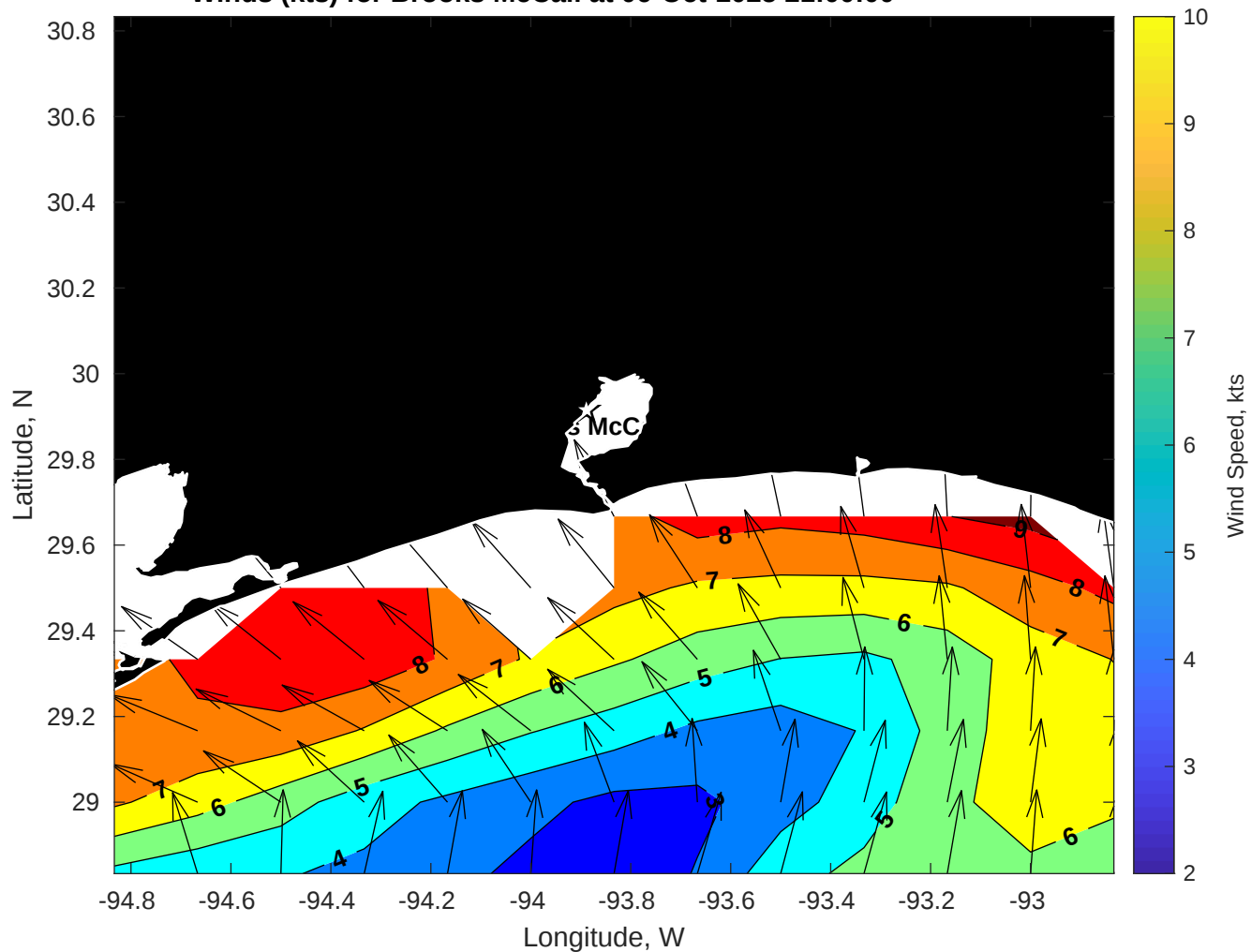
Winds (kts) for Brooks McCall at 06-Oct-2025 21:00:00
