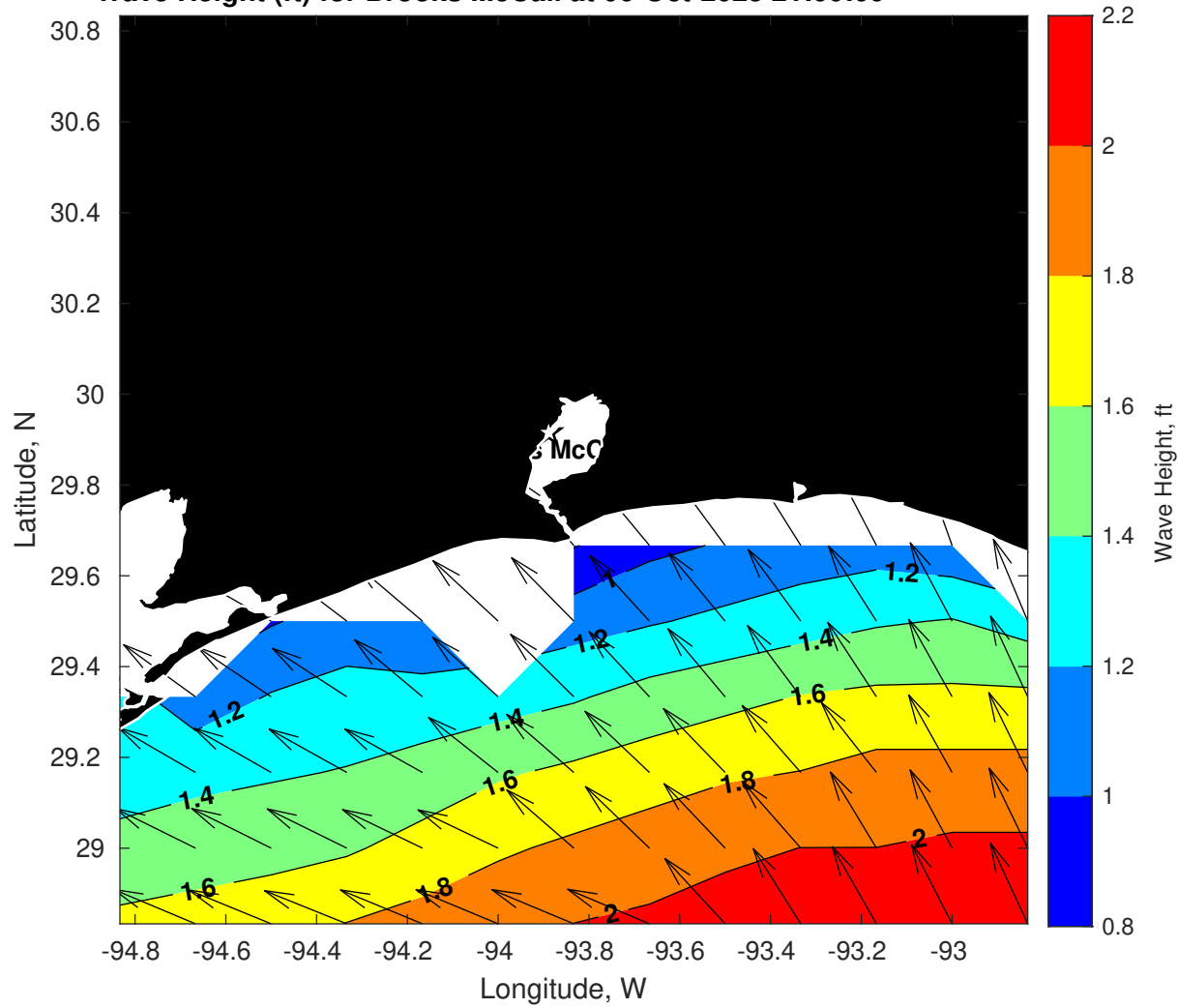
Wave Height (ft) for Brooks McCall at 06-Oct-2025 21:00:00
