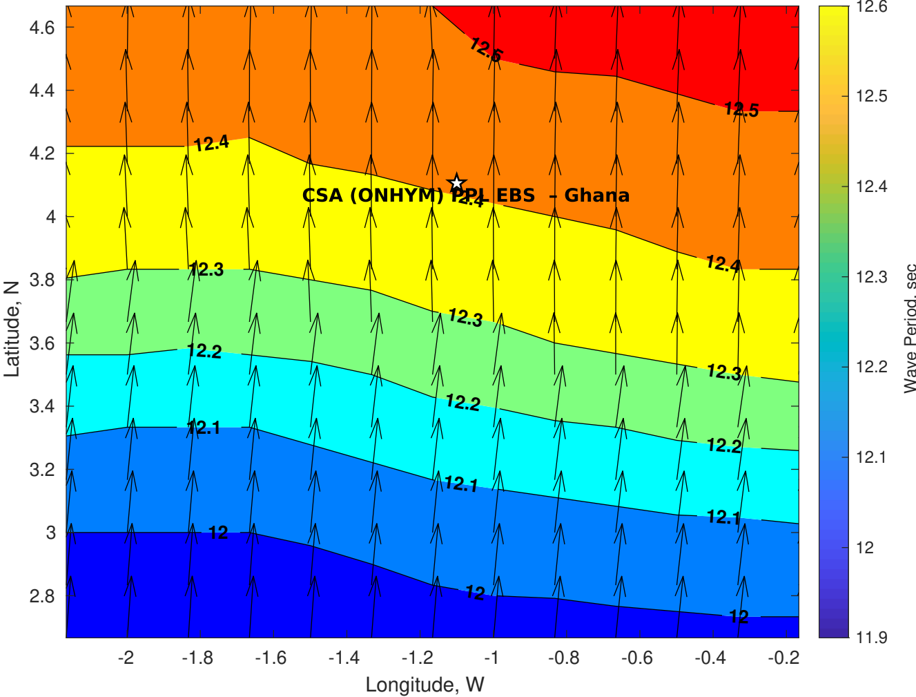
Wave Period (sec) for CSA (ONHYM) PPL EBS - Ghana at 06-Oct-2025 21:00:00
