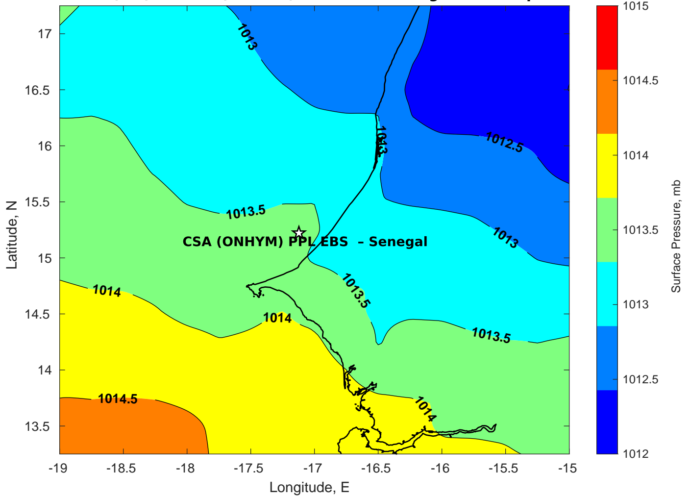
Surface Pressure (mb) for CSA (ONHYM) PPL EBS - Senegal at 19-Sep-2025 12:00:00
