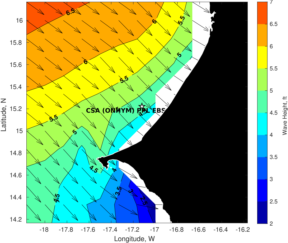
Wave Height (ft) for CSA (ONHYM) PPL EBS - Senegal at 06-Oct-2025 21:00:00
