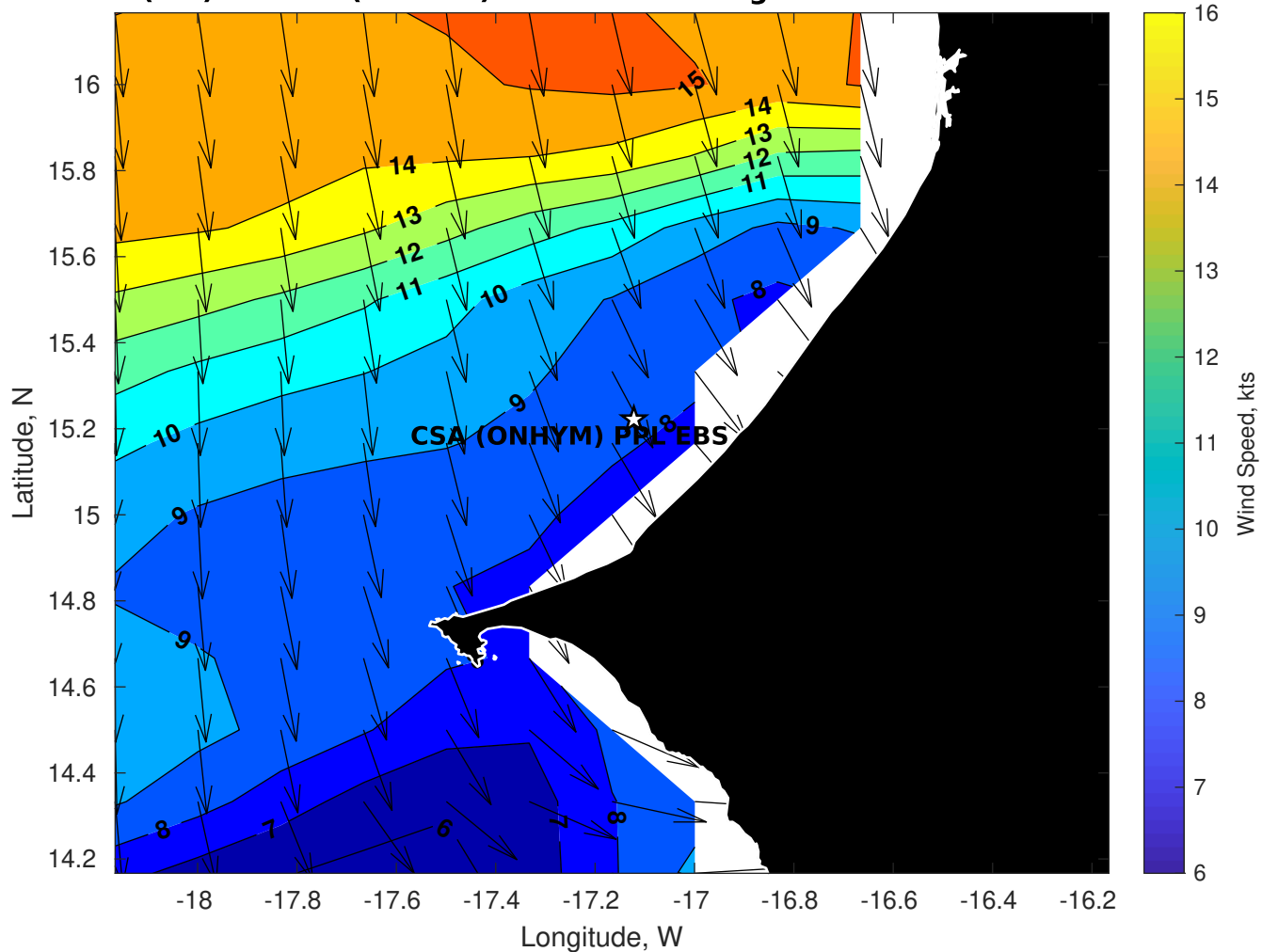
Winds (kts) for CSA (ONHYM) PPL EBS - Senegal at 06-Oct-2025 21:00:00
