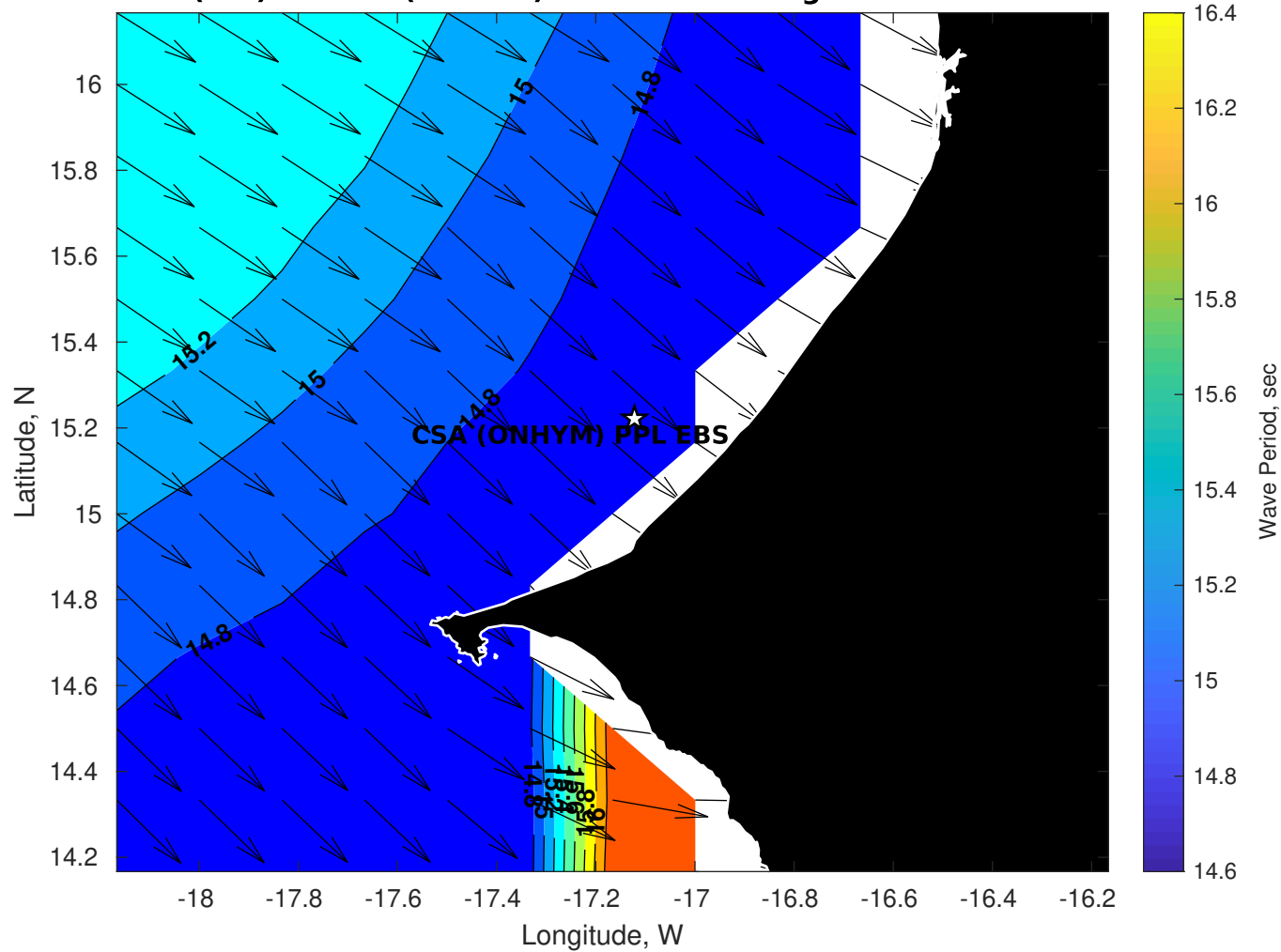
Wave Period (sec) for CSA (ONHYM) PPL EBS - Senegal at 06-Oct-2025 21:00:00
