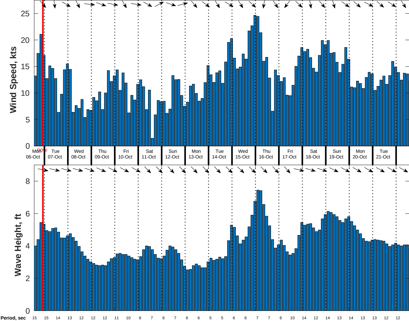
Wind & Wave Forecast for CSA (ONHYM) PPL EBS - Mauritania from 06-Oct-2025 13:00:00 to 22-Oct-2025 13:00:00
