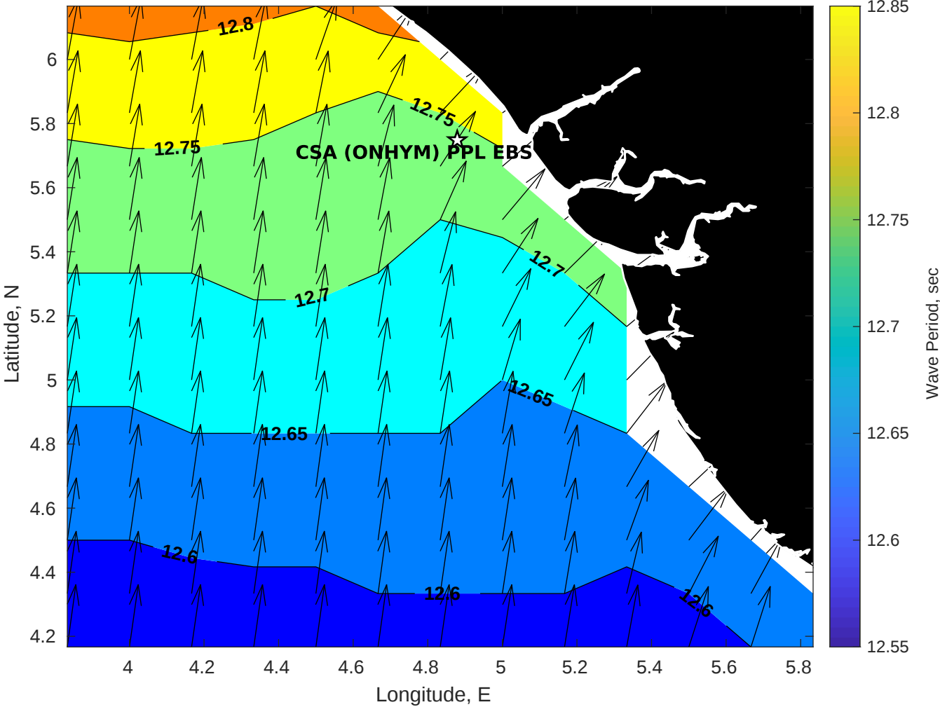
Wave Period (sec) for CSA (ONHYM) PPL EBS - Nigeria at 06-Oct-2025 21:00:00
