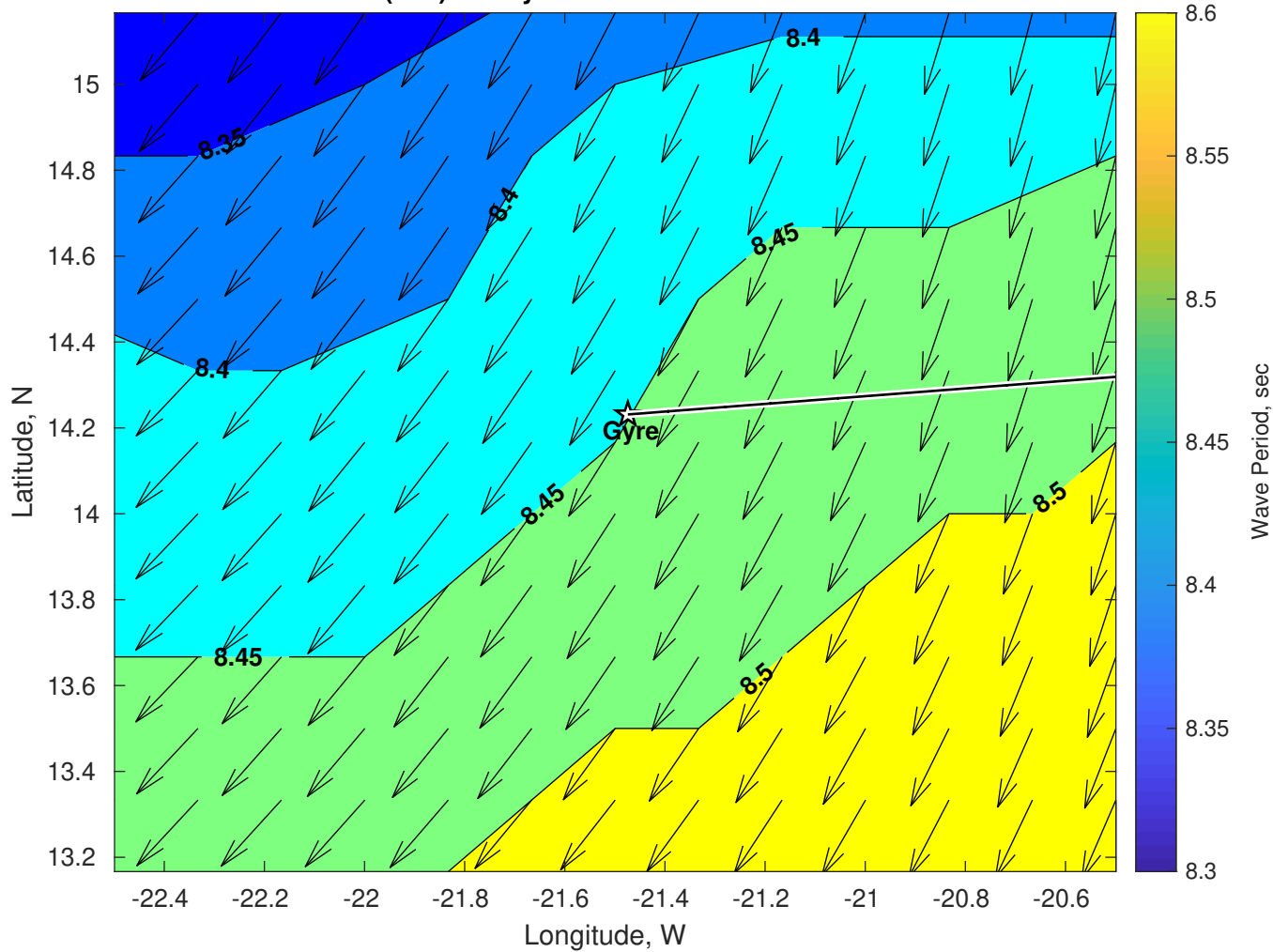
Wave Period (sec) for Gyre at 06-Oct-2025 21:00:00
