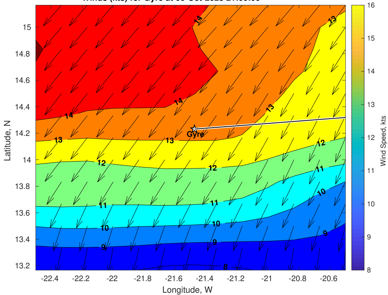
Winds (kts) for Gyre at 06-Oct-2025 21:00:00
