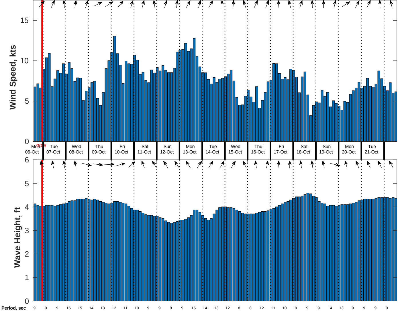
Wind & Wave Forecast for Nautilus from 06-Oct-2025 14:00:00 to 22-Oct-2025 14:00:00
