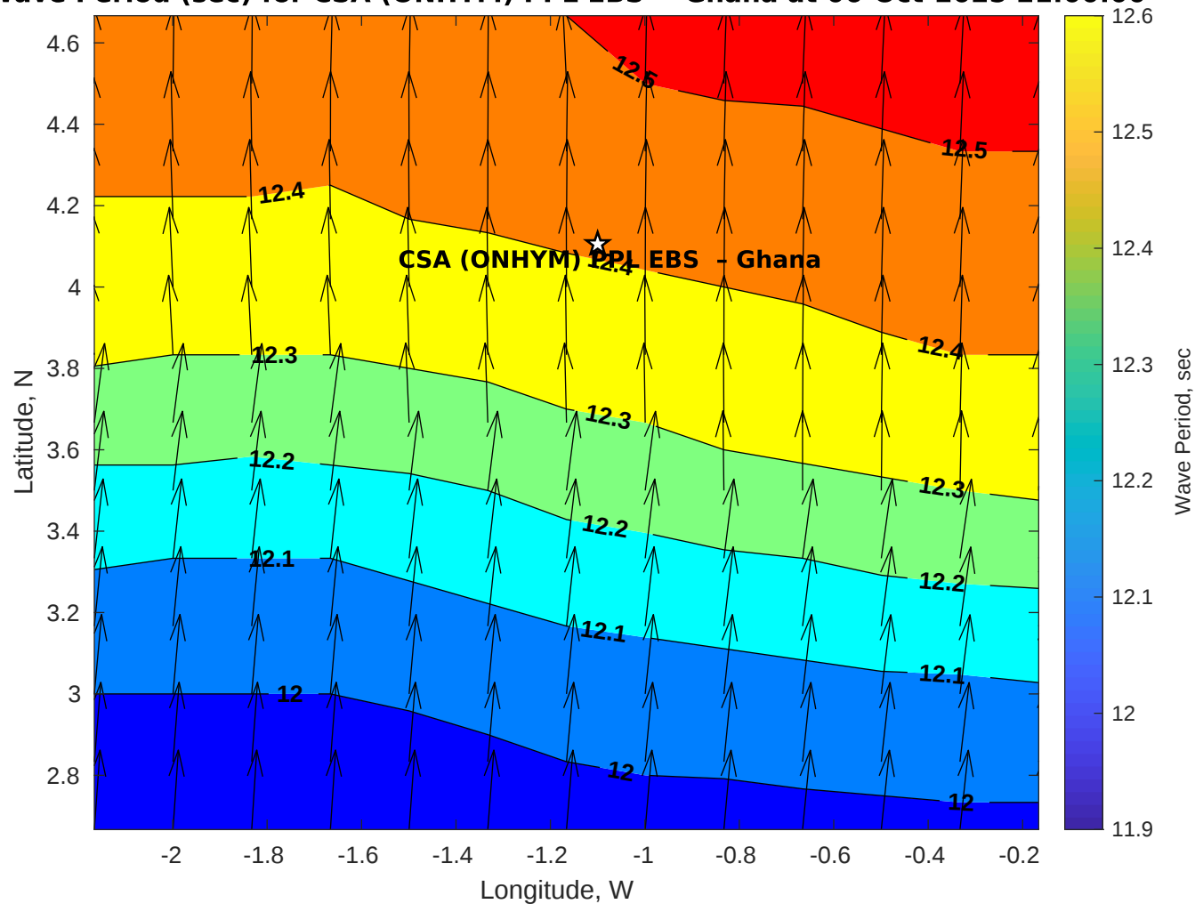
Wave Period (sec) for CSA (ONHYM) PPL EBS - Ghana at 06-Oct-2025 21:00:00
