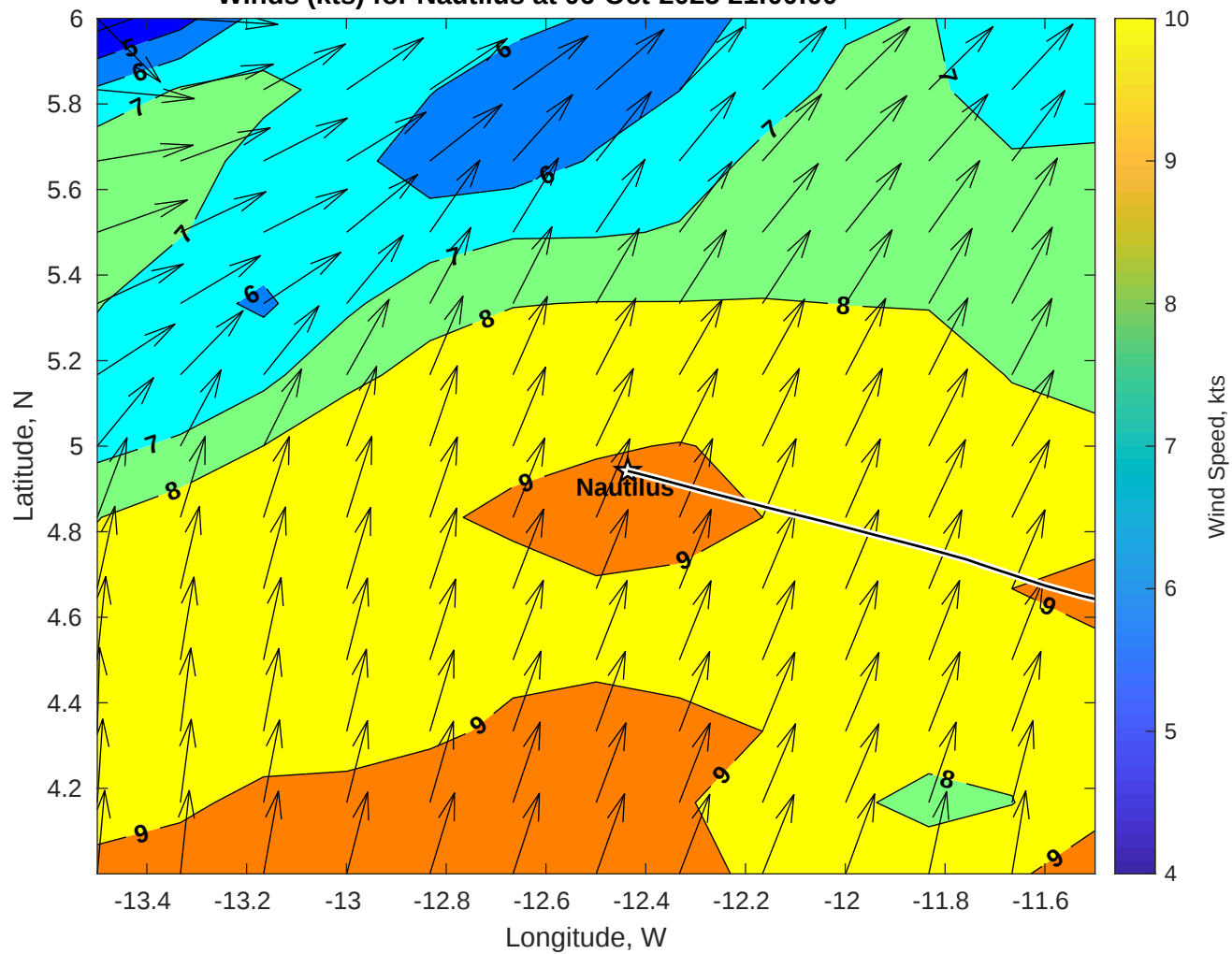
Winds (kts) for Nautilus at 06-Oct-2025 21:00:00
