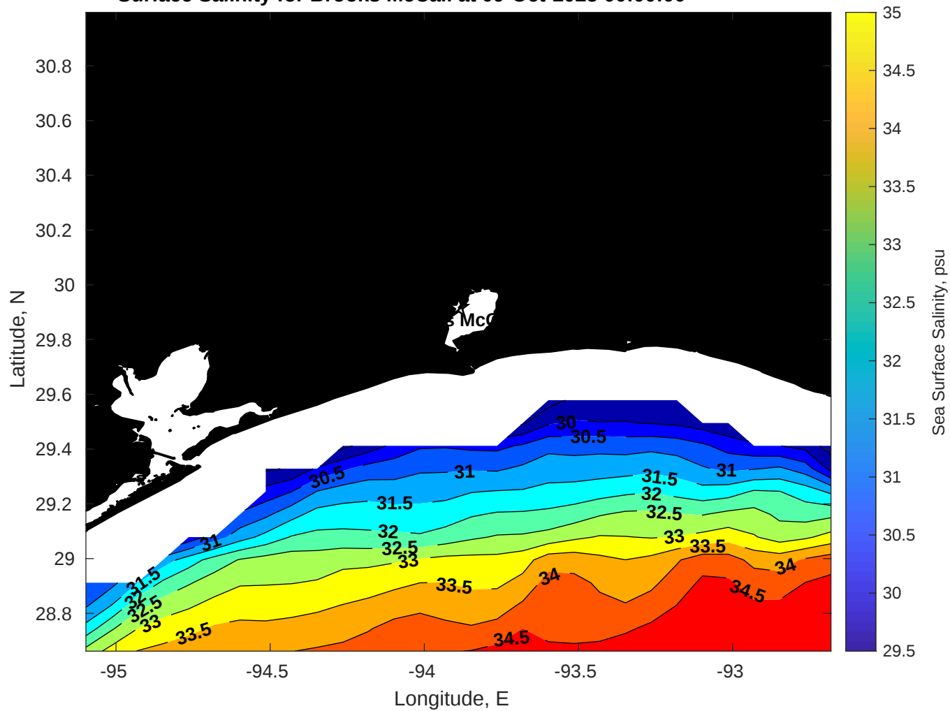
Surface Salinity for Brooks McCall at 09-Oct-2025 00:00:00
