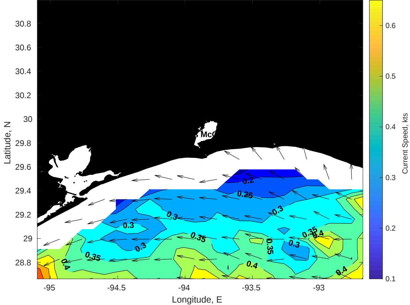
Surface Currents for Brooks McCall at 09-Oct-2025 00:00:00
