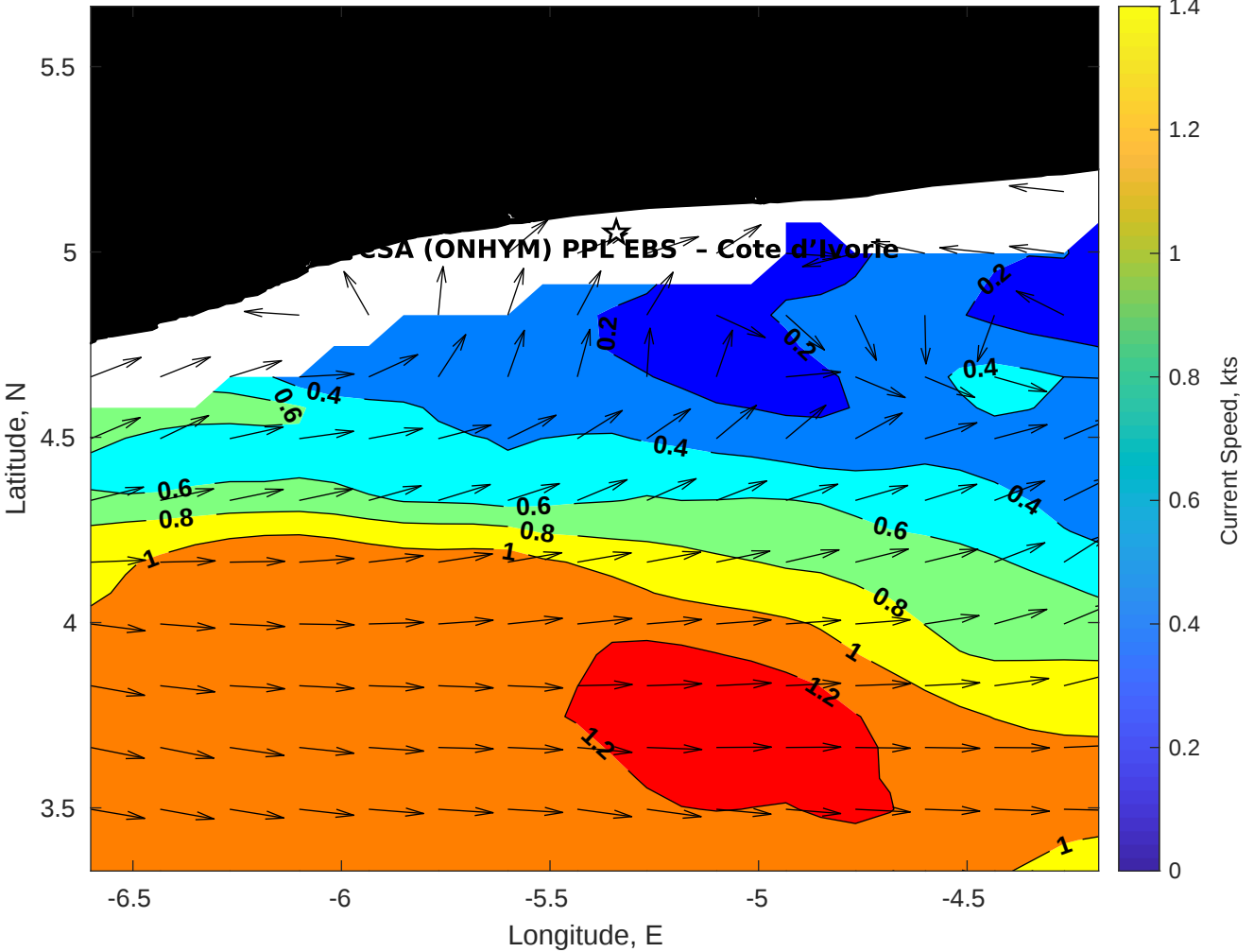
Surface Currents for CSA (ONHYM) PPL EBS - Cote d'Ivoire at 09-Oct-2025 00:00:00
