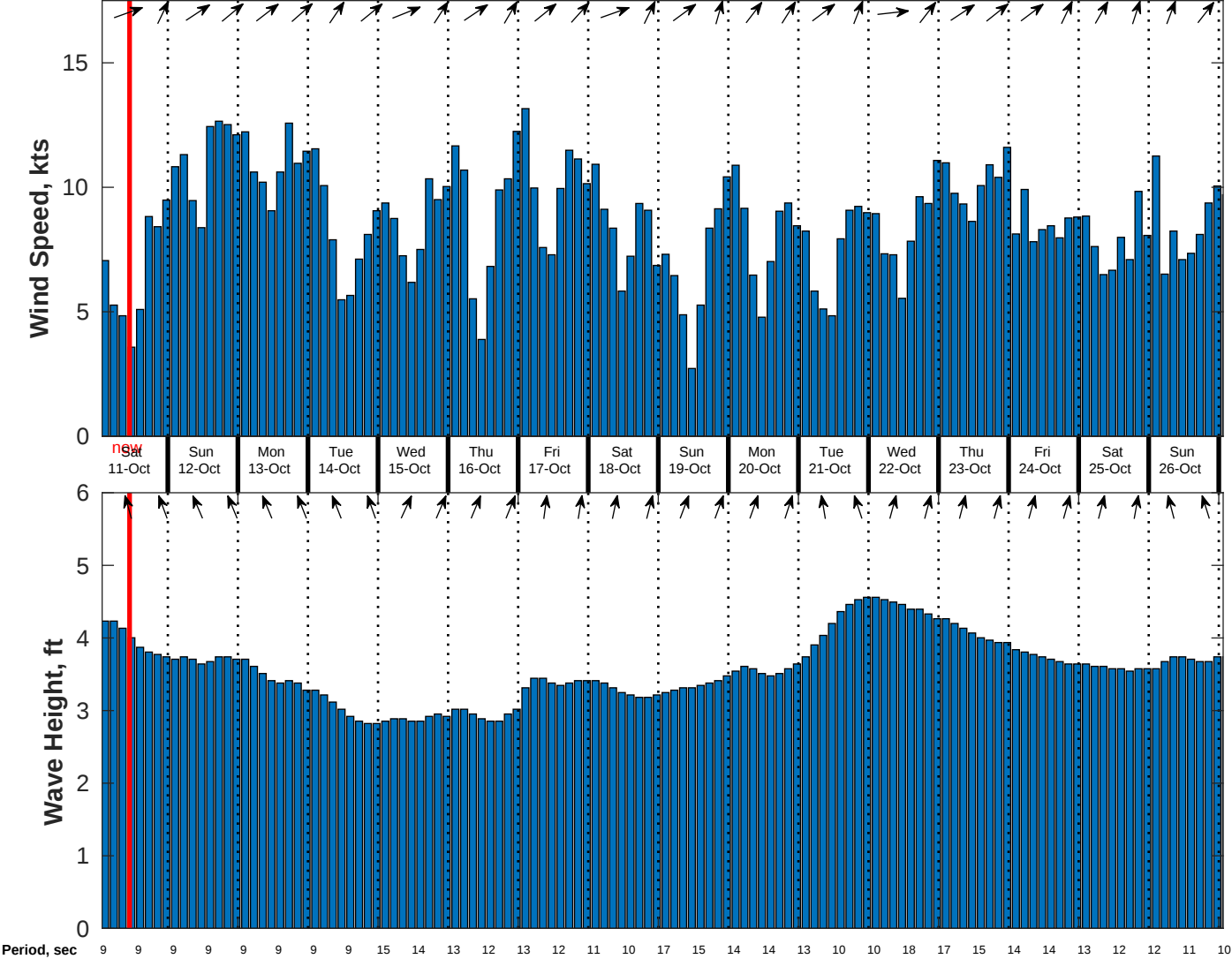
Wind & Wave Forecast for CSA (ONHYM) PPL EBS - Cote d'Ivoire from 10-Oct-2025 01:00:00 to 26-Oct-2025 01:00:00
