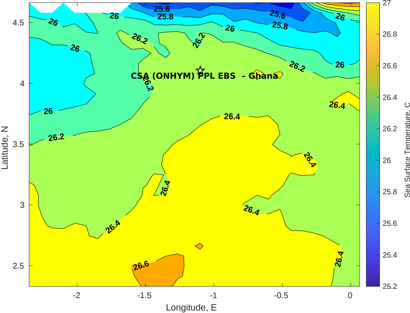
SST for CSA (ONHYM) PPL EBS - Ghana at 09-Oct-2025 00:00:00
