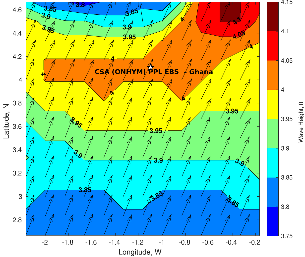
Wave Height (ft) for CSA (ONHYM) PPL EBS - Ghana at 10-Oct-2025 09:00:00
