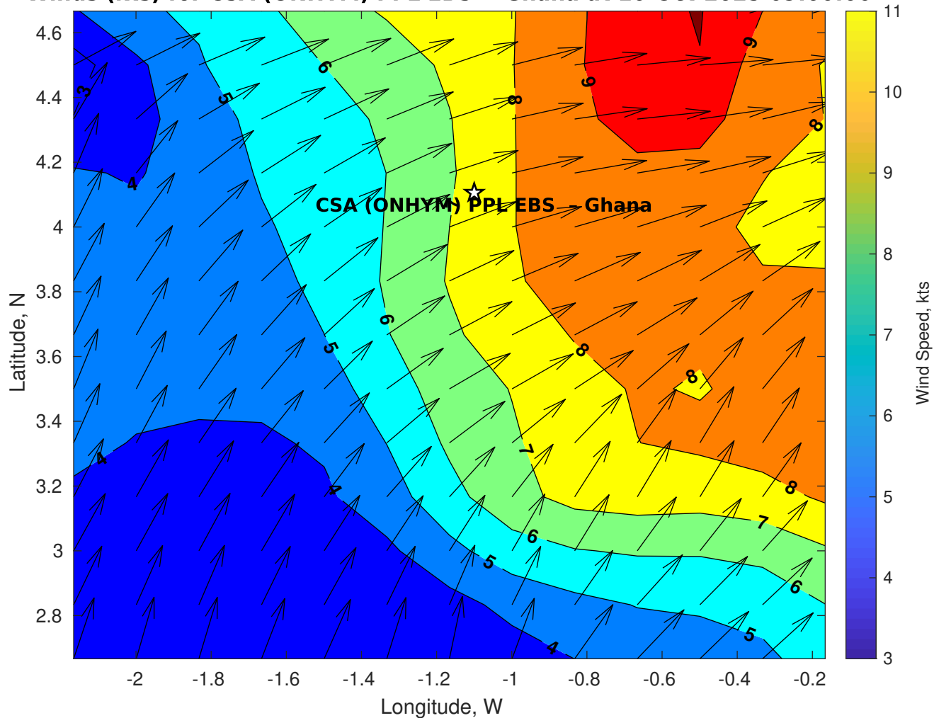
Winds (kts) for CSA (ONHYM) PPL EBS - Ghana at 10-Oct-2025 09:00:00
