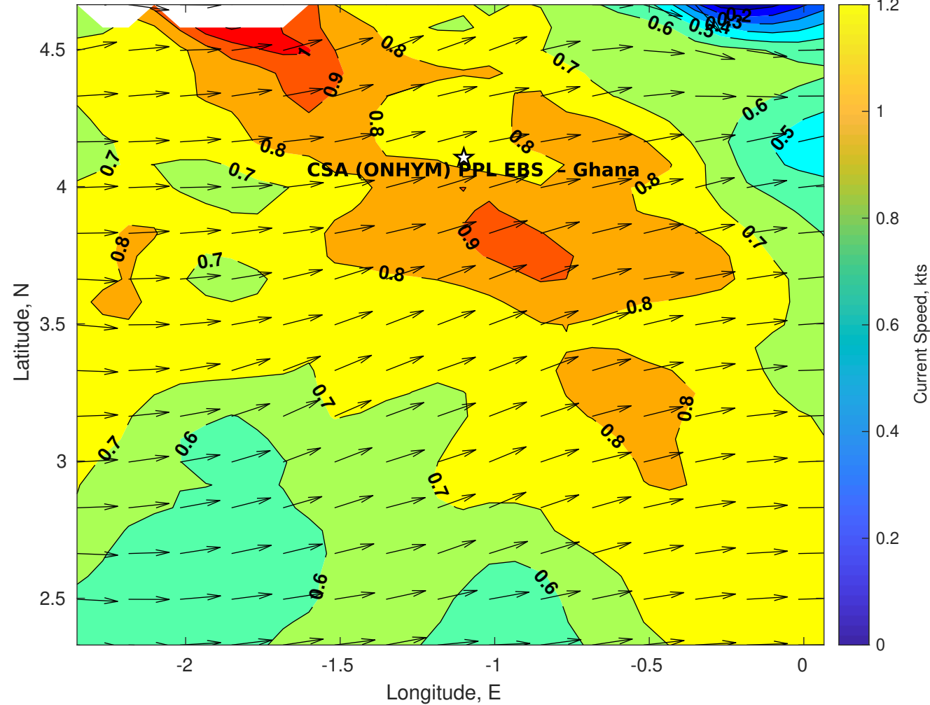
Surface Currents for CSA (ONHYM) PPL EBS - Ghana at 09-Oct-2025 00:00:00
