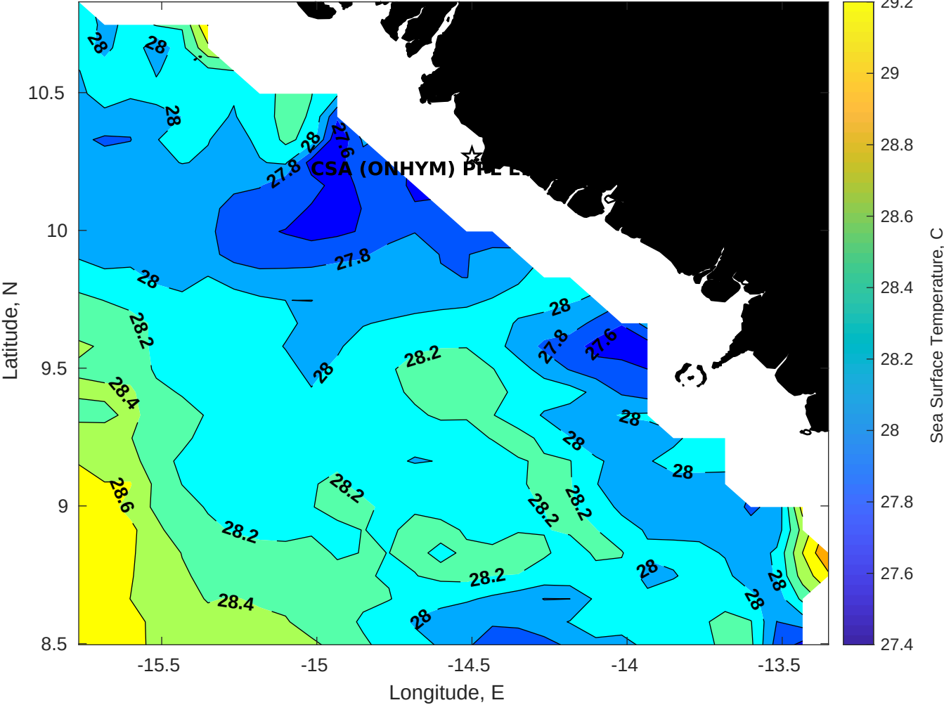
SST for CSA (ONHYM) PPL EBS - Guinea at 09-Oct-2025 00:00:00
