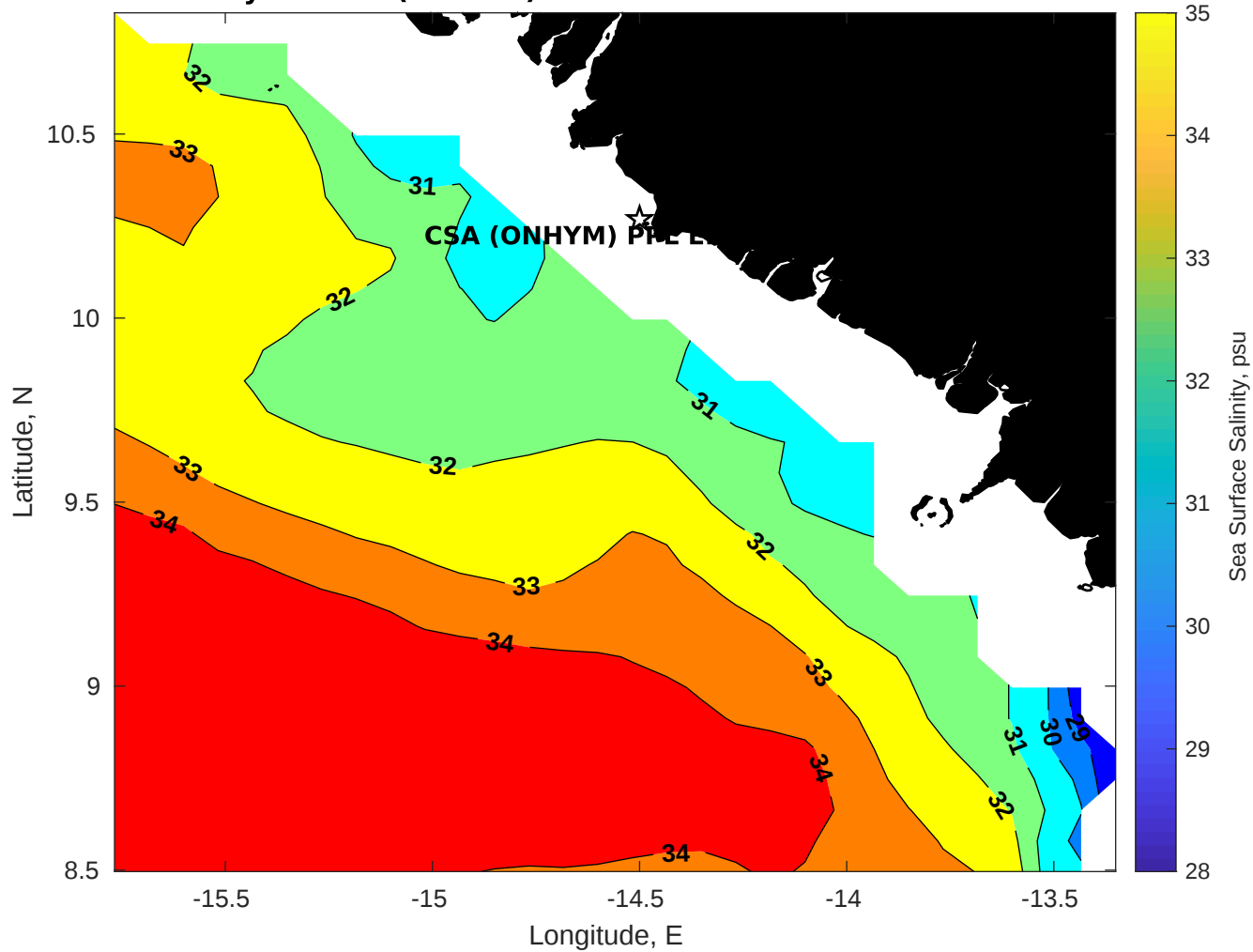
Surface Salinity for CSA (ONHYM) PPL EBS - Guinea at 09-Oct-2025 00:00:00
