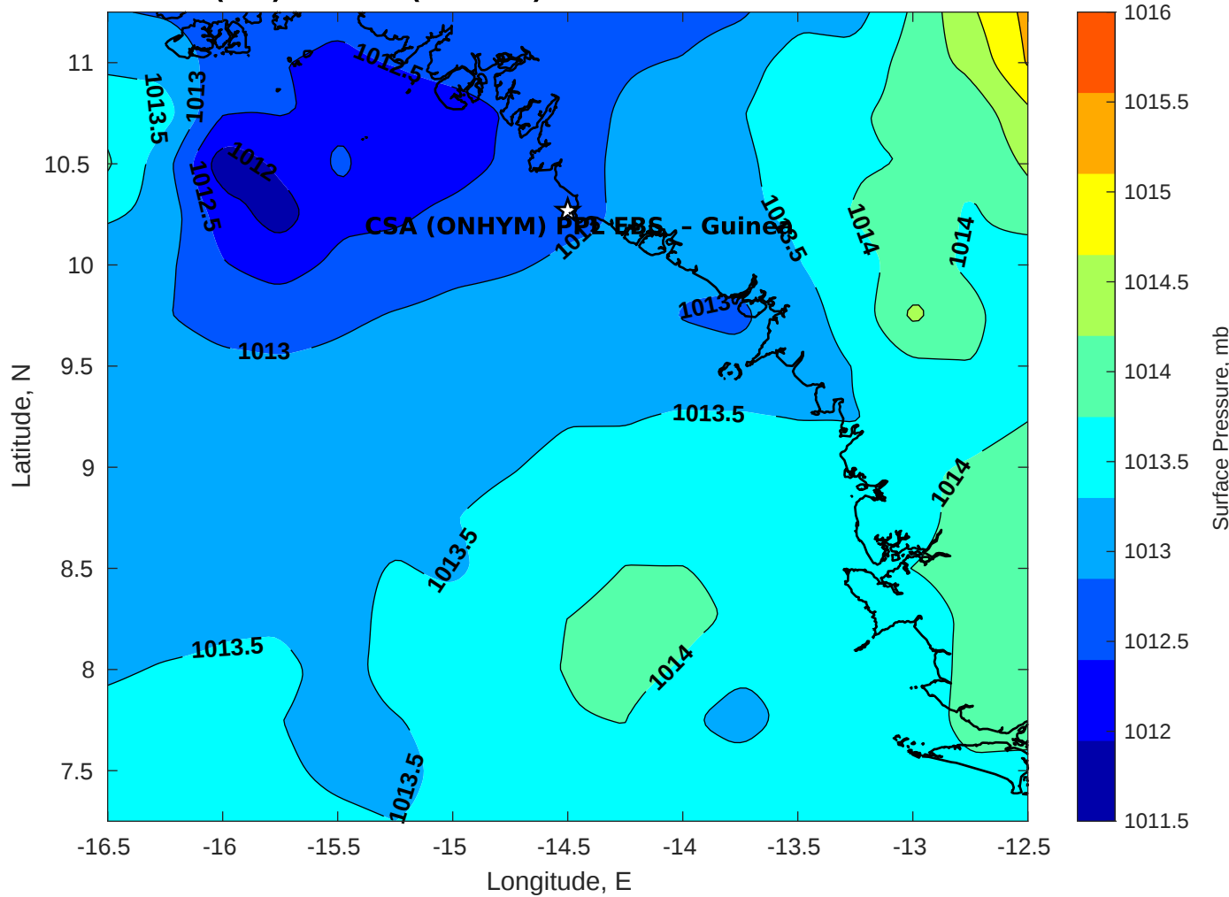
Surface Pressure (mb) for CSA (ONHYM) PPL EBS - Guinea at 10-Oct-2025 00:00:00
