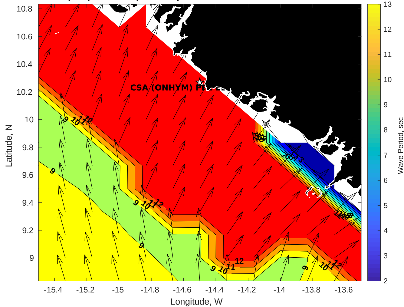
Wave Period (sec) for CSA (ONHYM) PPL EBS - Guinea at 10-Oct-2025 09:00:00
