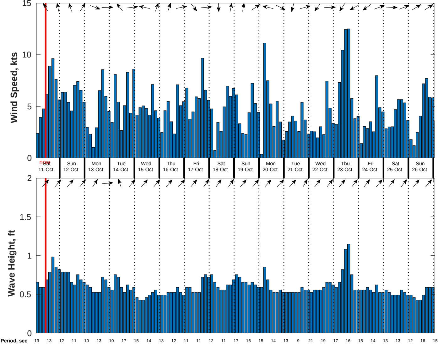
Wind & Wave Forecast for CSA (ONHYM) PPL EBS - Guinea from 10-Oct-2025 01:00:00 to 26-Oct-2025 01:00:00
