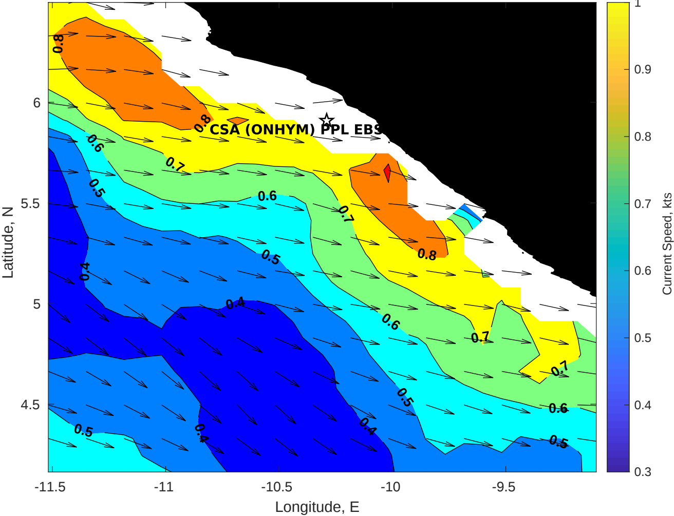
Surface Currents for CSA (ONHYM) PPL EBS - Liberia at 09-Oct-2025 00:00:00
