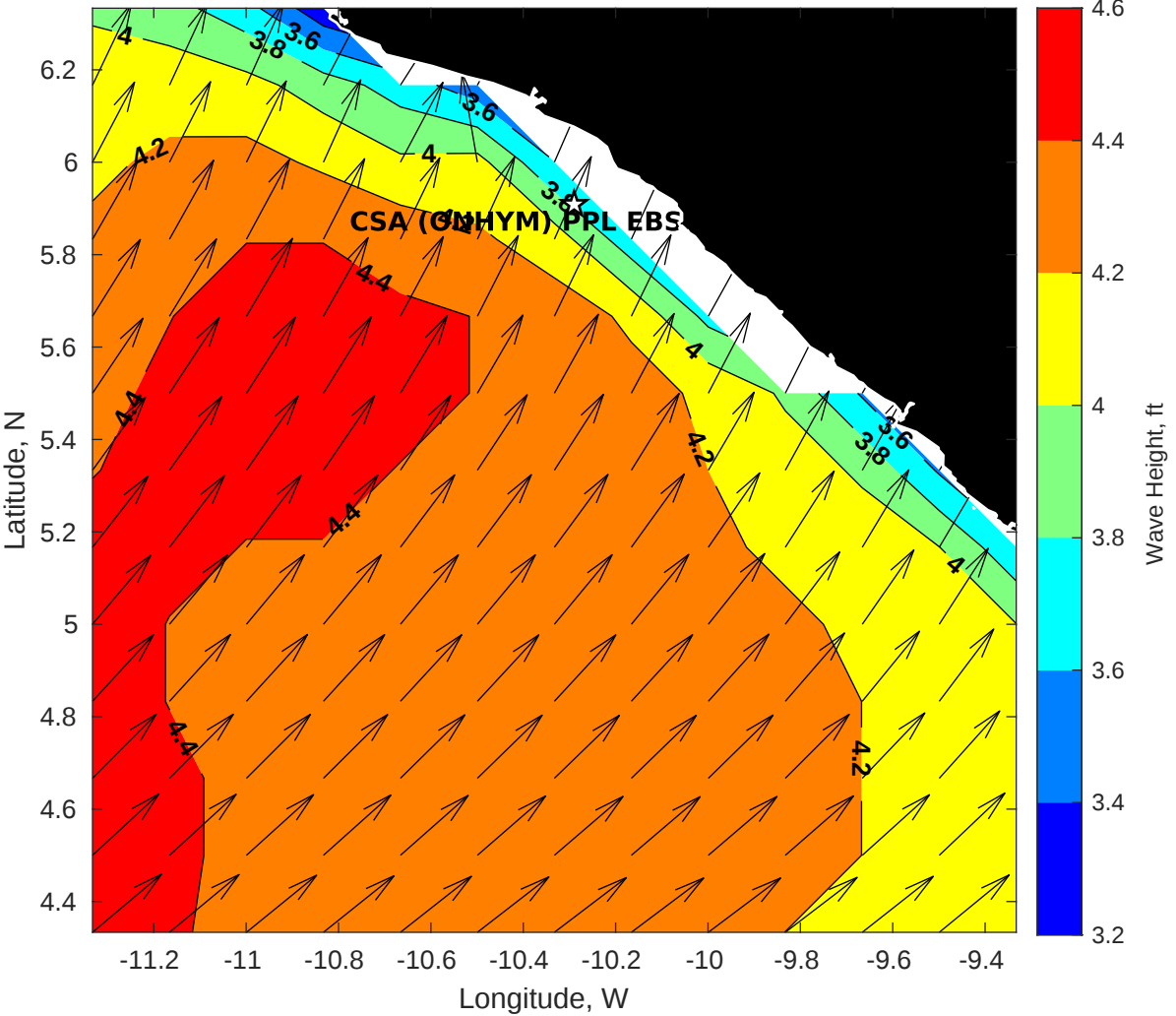
Wave Height (ft) for CSA (ONHYM) PPL EBS - Liberia at 10-Oct-2025 09:00:00
