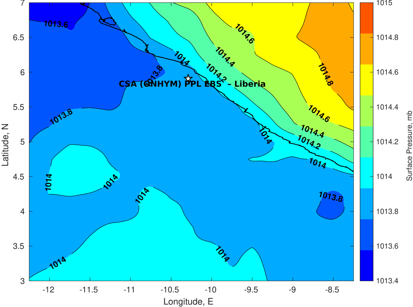
Surface Pressure (mb) for CSA (ONHYM) PPL EBS - Liberia at 10-Oct-2025 00:00:00
