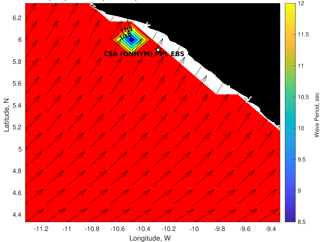
Wave Period (sec) for CSA (ONHYM) PPL EBS - Liberia at 10-Oct-2025 09:00:00
