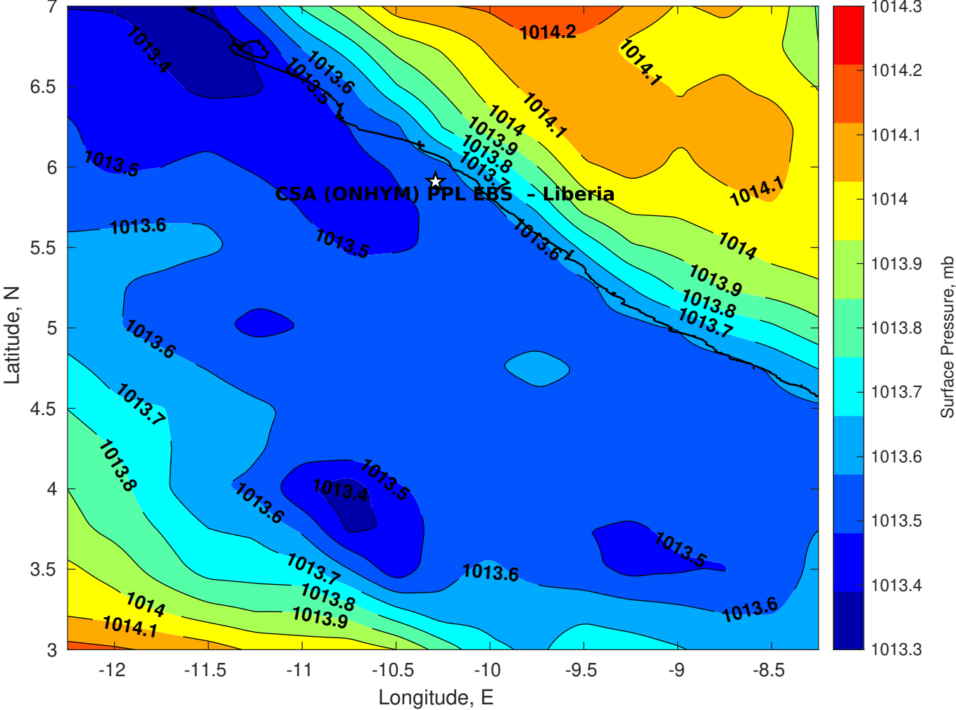
Surface Pressure (mb) for CSA (ONHYM) PPL EBS - Liberia at 11-Oct-2025 00:00:00
