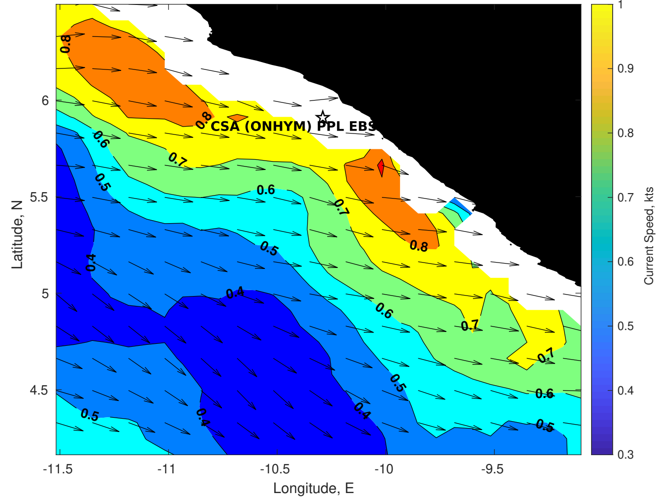
Surface Currents for CSA (ONHYM) PPL EBS - Liberia at 09-Oct-2025 00:00:00
