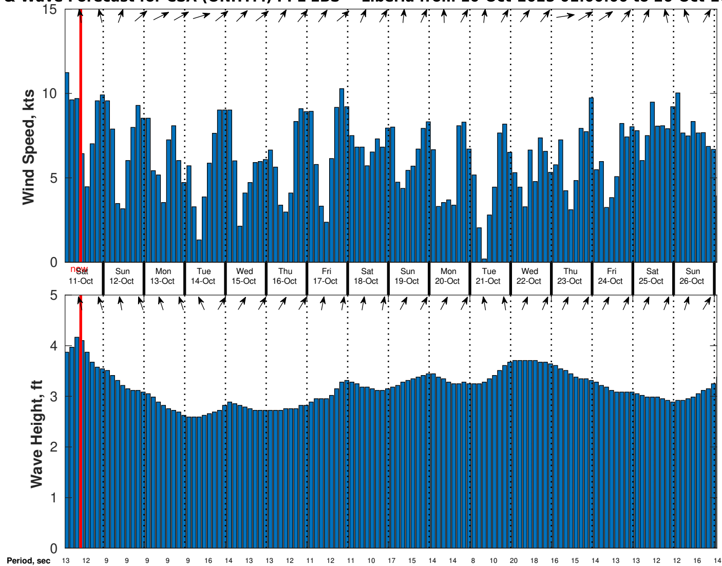
Wind & Wave Forecast for CSA (ONHYM) PPL EBS - Liberia from 10-Oct-2025 01:00:00 to 26-Oct-2025 01:00:00
