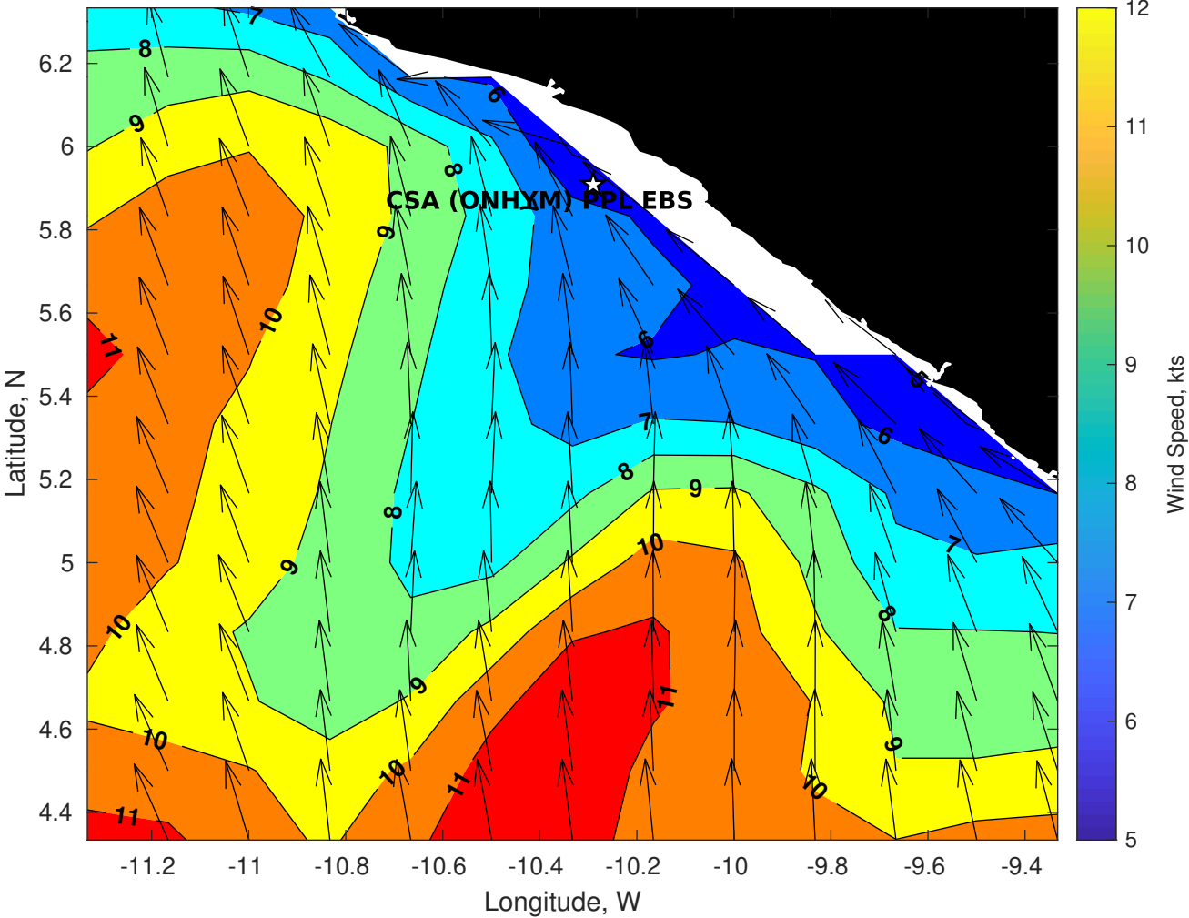
Winds (kts) for CSA (ONHYM) PPL EBS - Liberia at 10-Oct-2025 09:00:00
