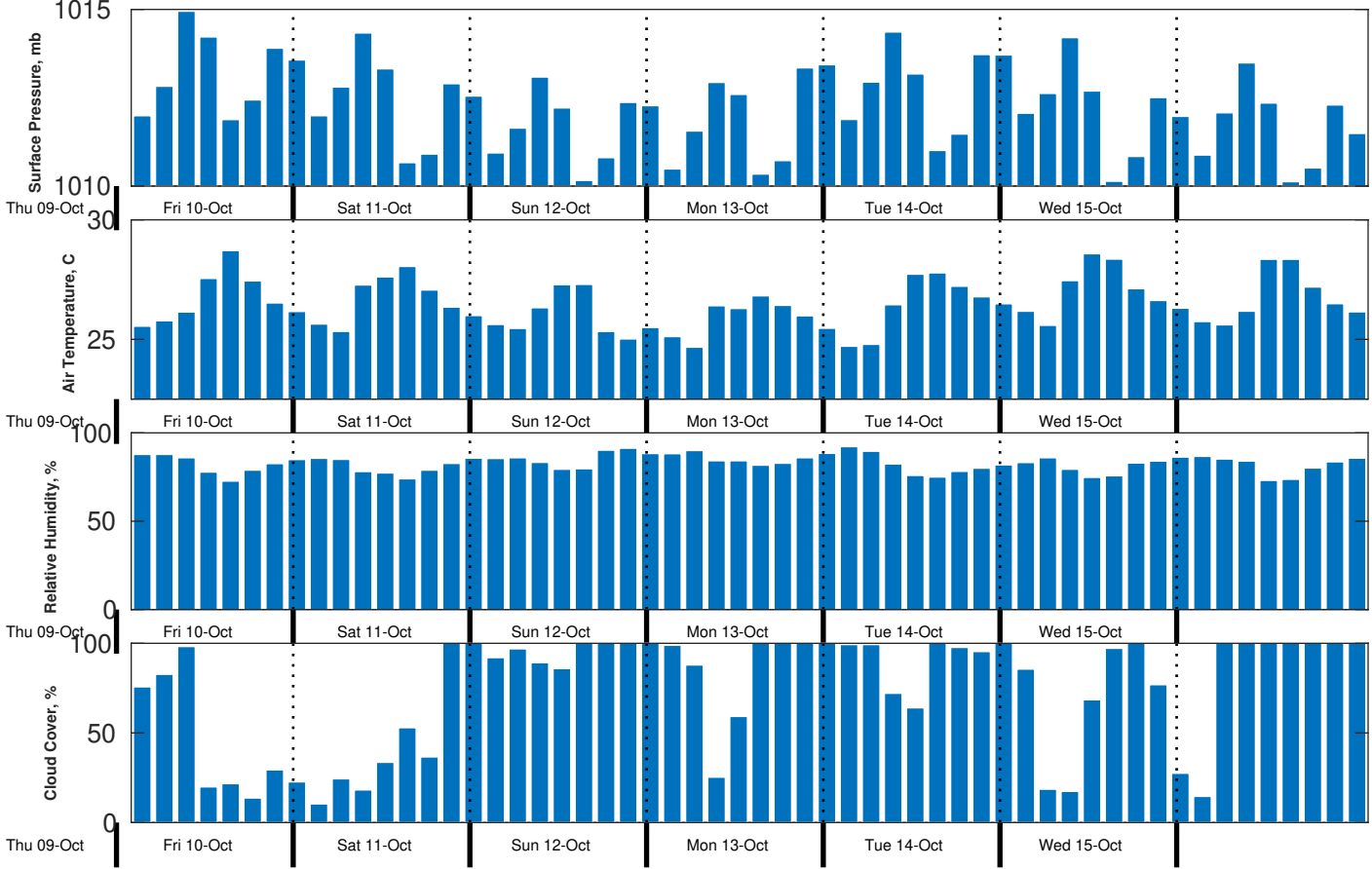
Met Forecast for CSA (ONHYM) PPL EBS - Liberia from 10-Oct-2025 00:00:00 to 17-Oct-2025 00:00:00
