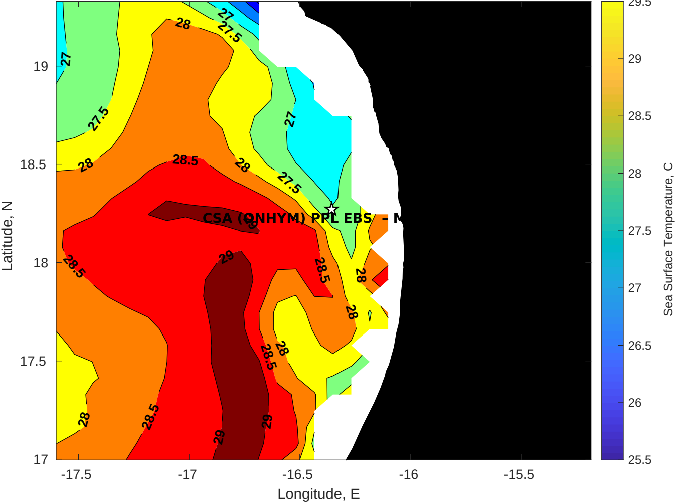
SST for CSA (ONHYM) PPL EBS - Mauritania at 09-Oct-2025 00:00:00
