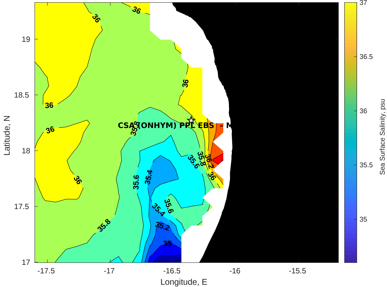
Surface Salinity for CSA (ONHYM) PPL EBS - Mauritania at 09-Oct-2025 00:00:00
