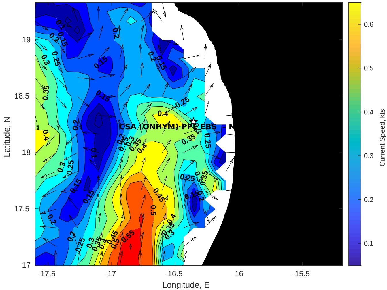
Surface Currents for CSA (ONHYM) PPL EBS - Mauritania at 09-Oct-2025 00:00:00
