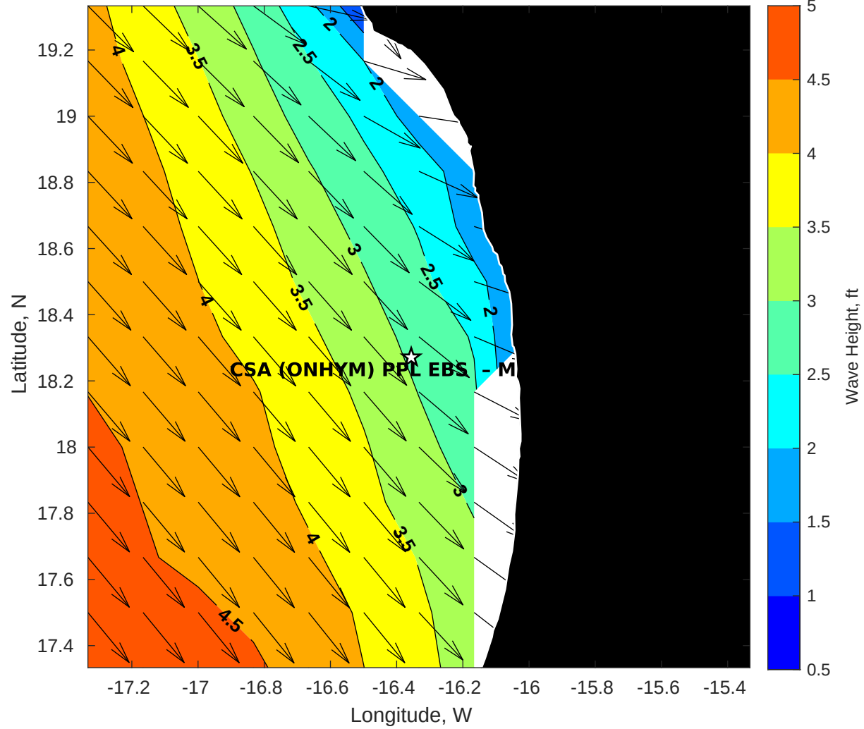
Wave Height (ft) for CSA (ONHYM) PPL EBS - Mauritania at 10-Oct-2025 09:00:00
