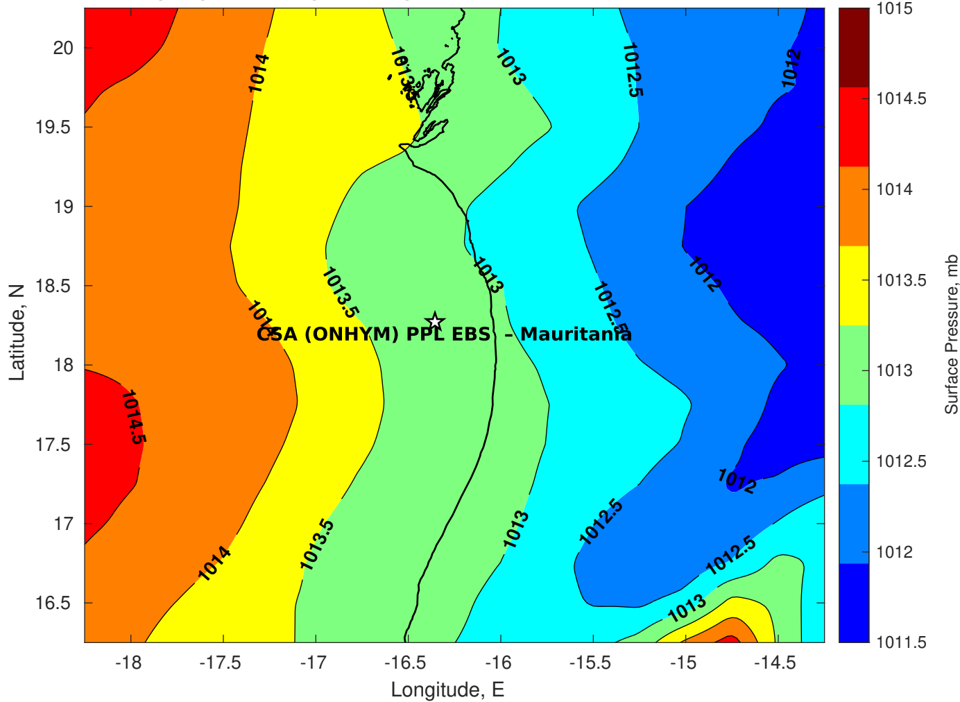
Surface Pressure (mb) for CSA (ONHYM) PPL EBS - Mauritania at 10-Oct-2025 00:00:00
