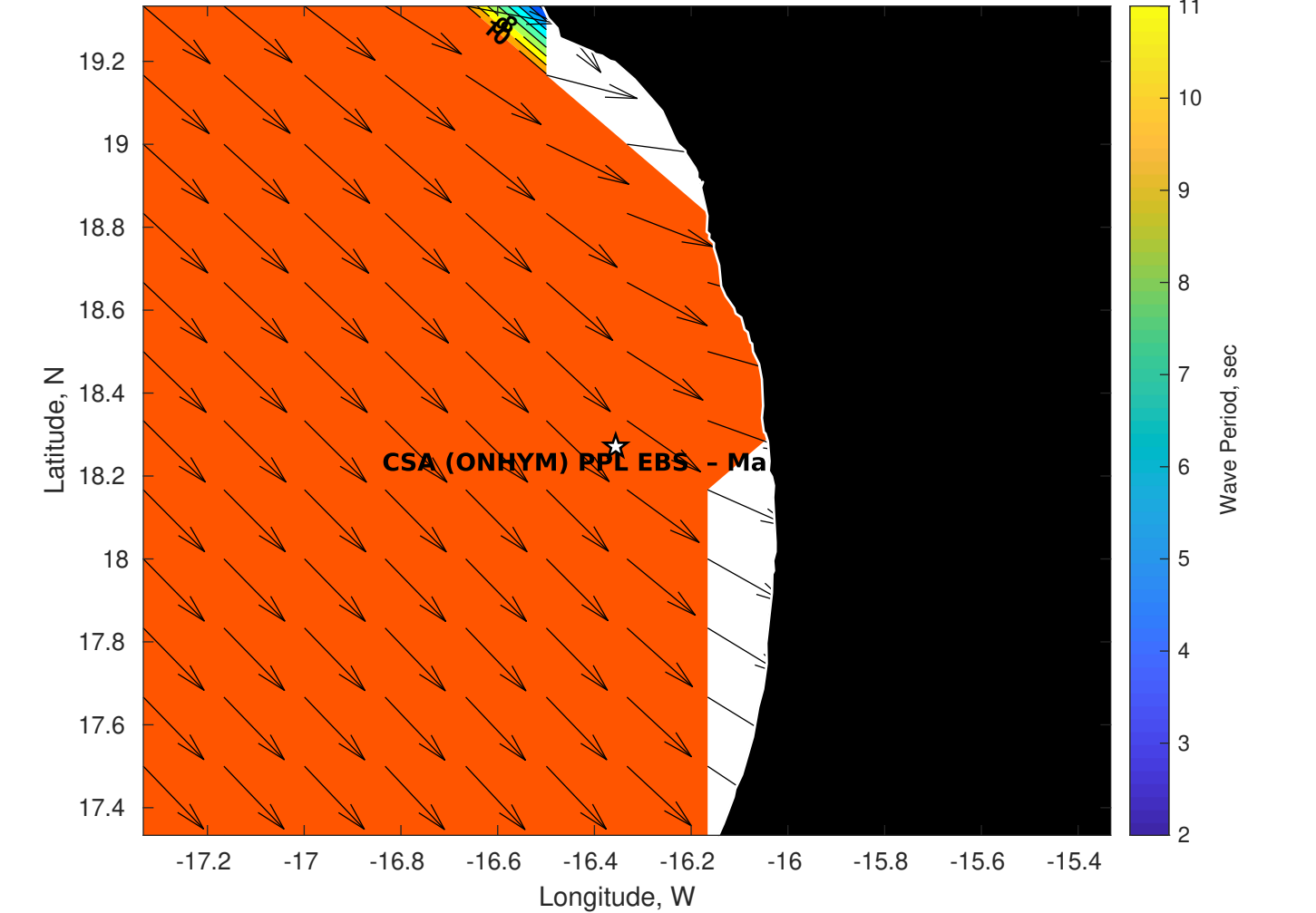
Wave Period (sec) for CSA (ONHYM) PPL EBS - Mauritania at 10-Oct-2025 09:00:00
