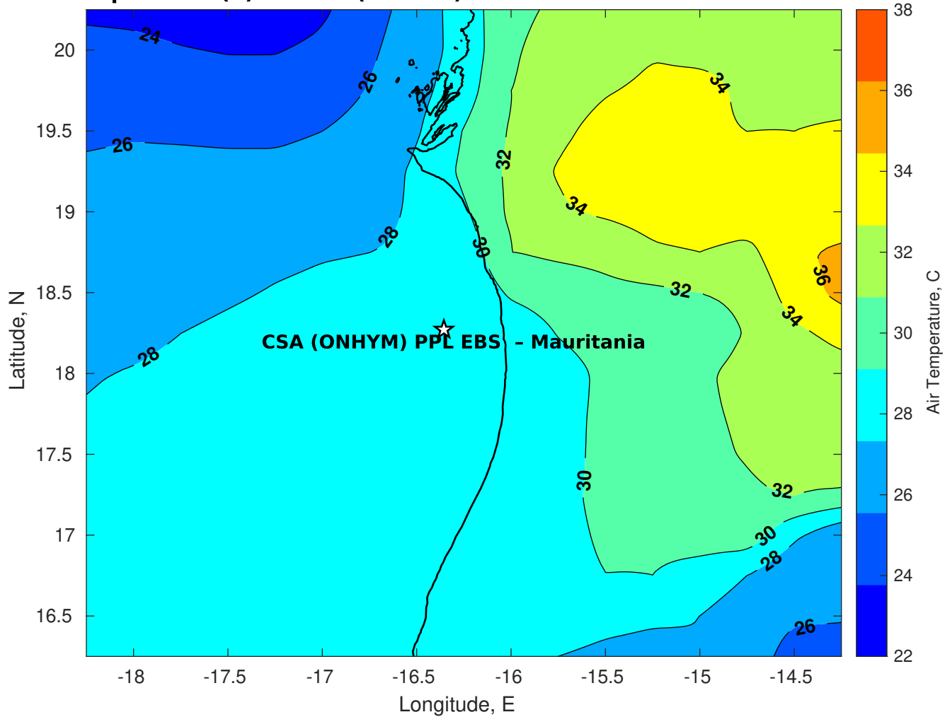
Air Temperature (C) for CSA (ONHYM) PPL EBS - Mauritania at 10-Oct-2025
