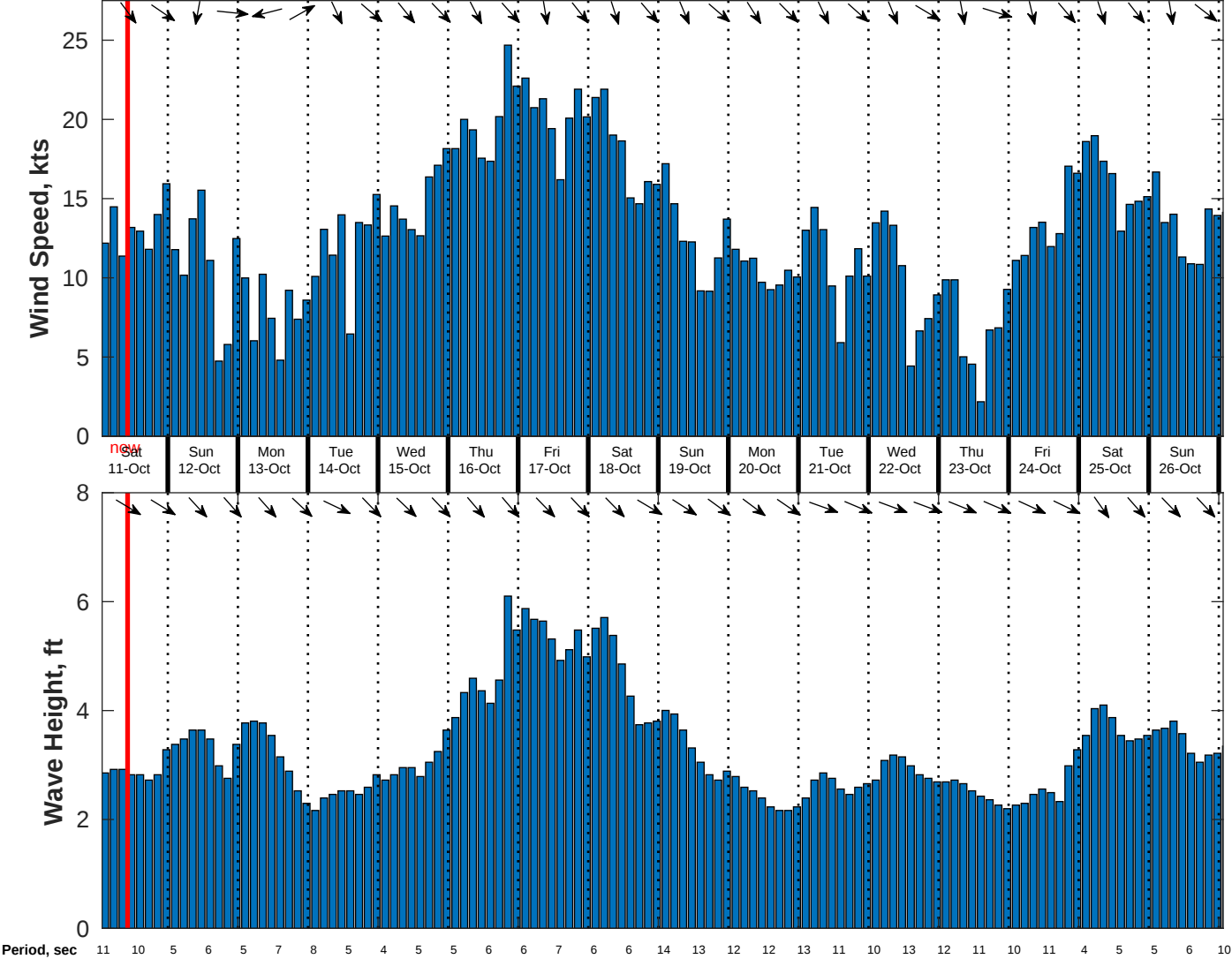
Wind & Wave Forecast for CSA (ONHYM) PPL EBS - Mauritania from 10-Oct-2025 01:00:00 to 26-Oct-2025 01:00:00
