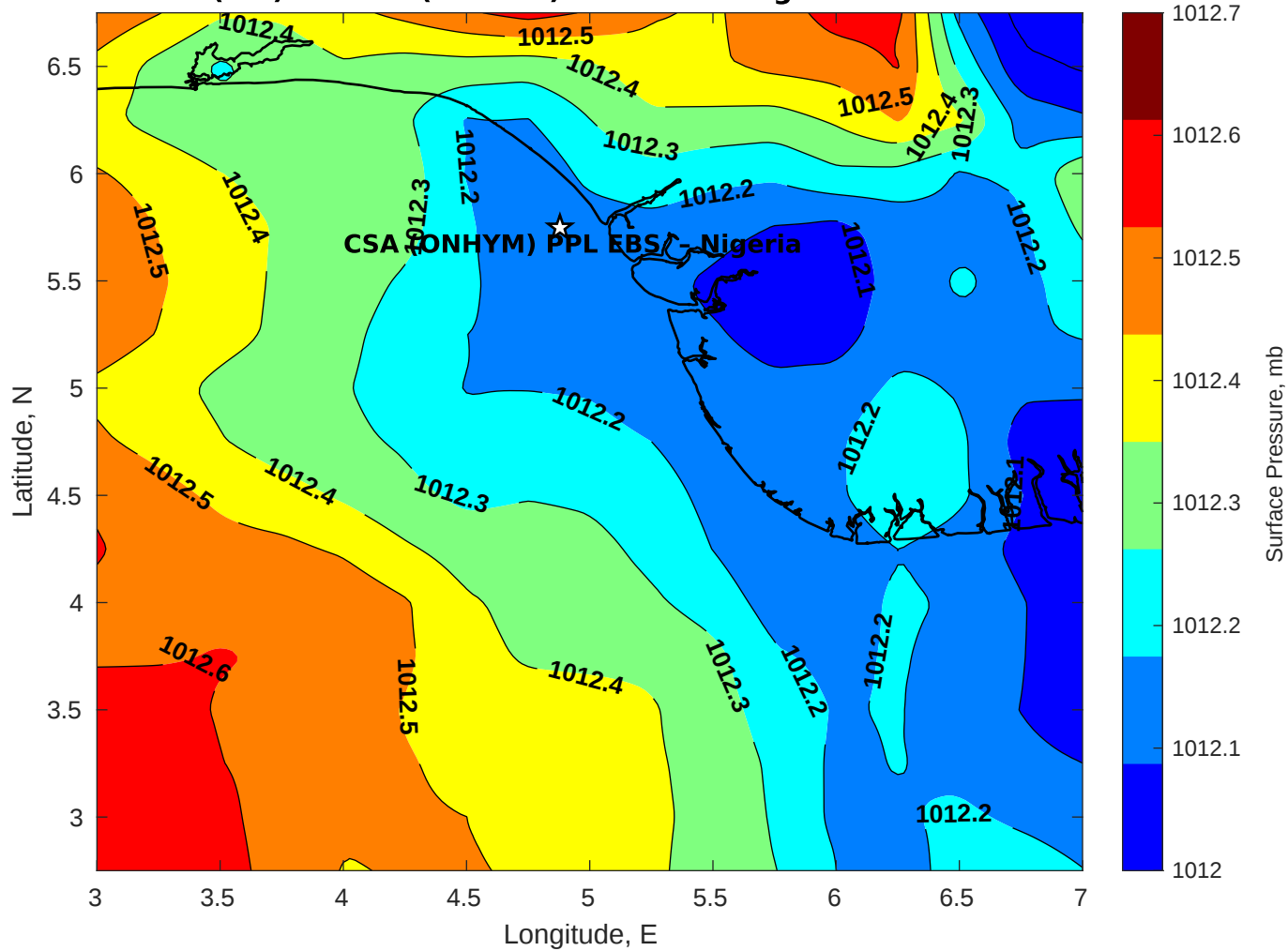
Surface Pressure (mb) for CSA (ONHYM) PPL EBS - Nigeria at 10-Oct-2025 00:00:00
