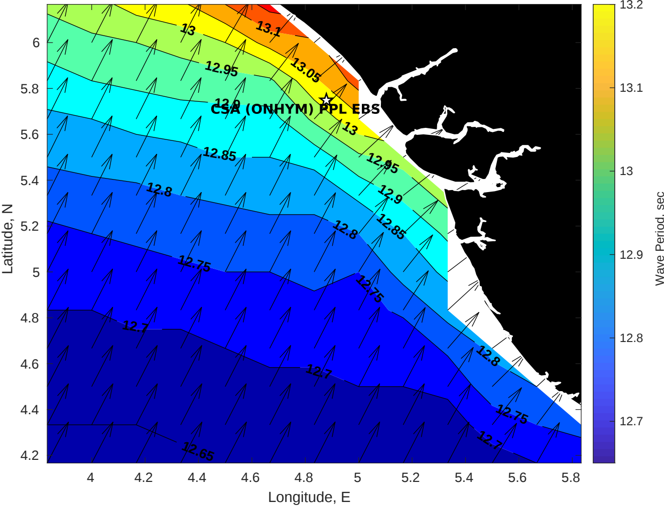
Wave Period (sec) for CSA (ONHYM) PPL EBS - Nigeria at 10-Oct-2025 09:00:00
