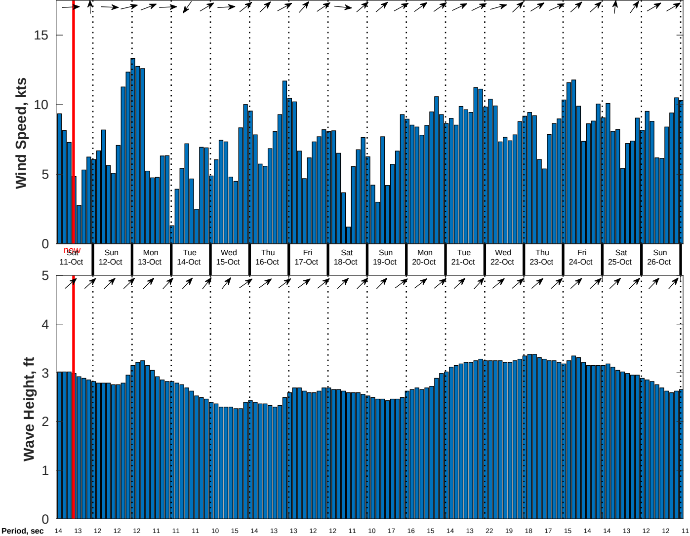
Wind & Wave Forecast for CSA (ONHYM) PPL EBS - Nigeria from 10-Oct-2025 02:00:00 to 26-Oct-2025 02:00:00
